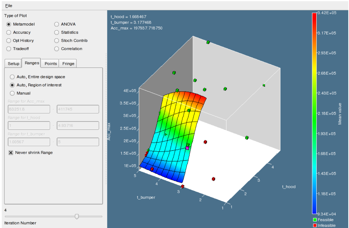
Figure 18-3: Surface plot representing only the region of interest of the fourth iteration.
