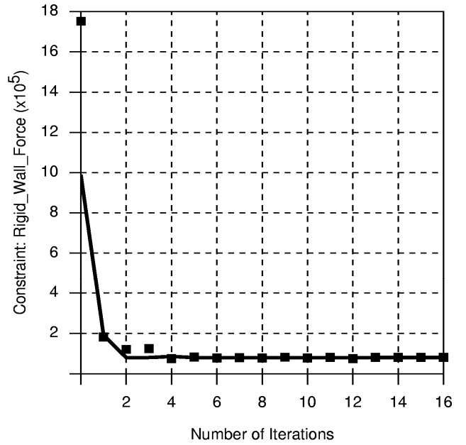
d) Rigid_Wall_Force
