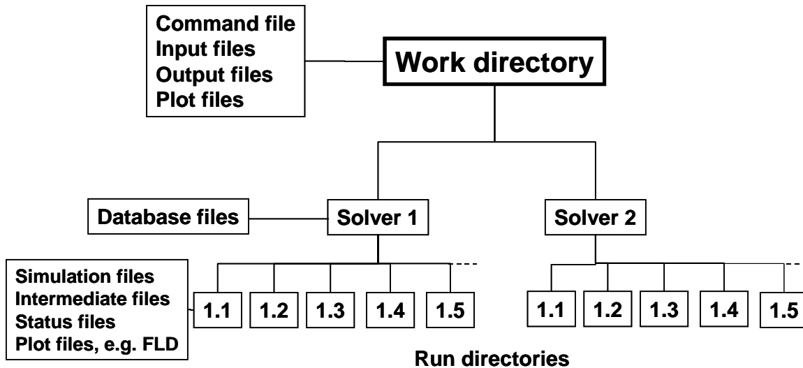
Figure 9-1 : Directory structure in LS-OPT
