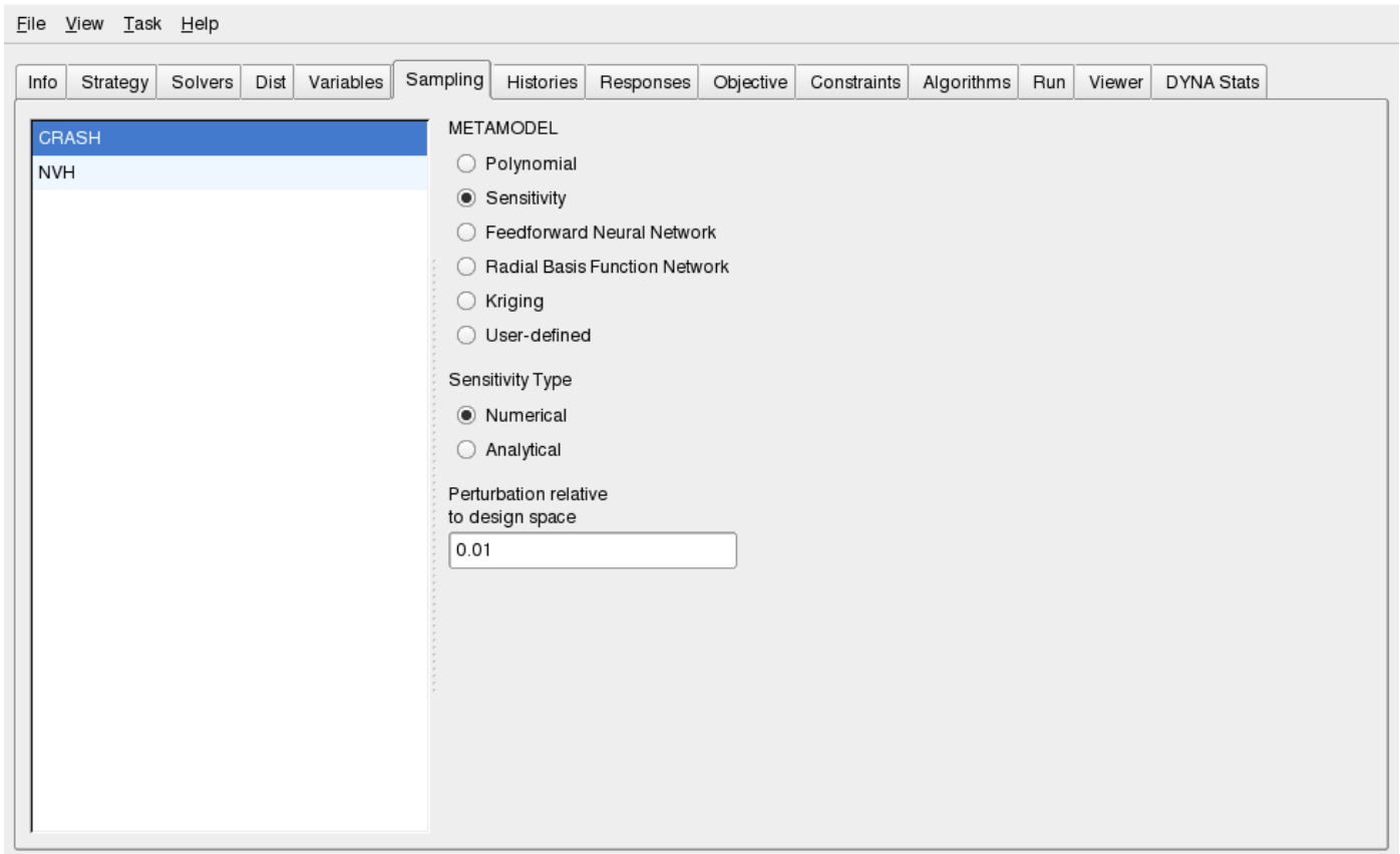
Figure 13-3: Selecting Sensitivities in the Point Selection panel
