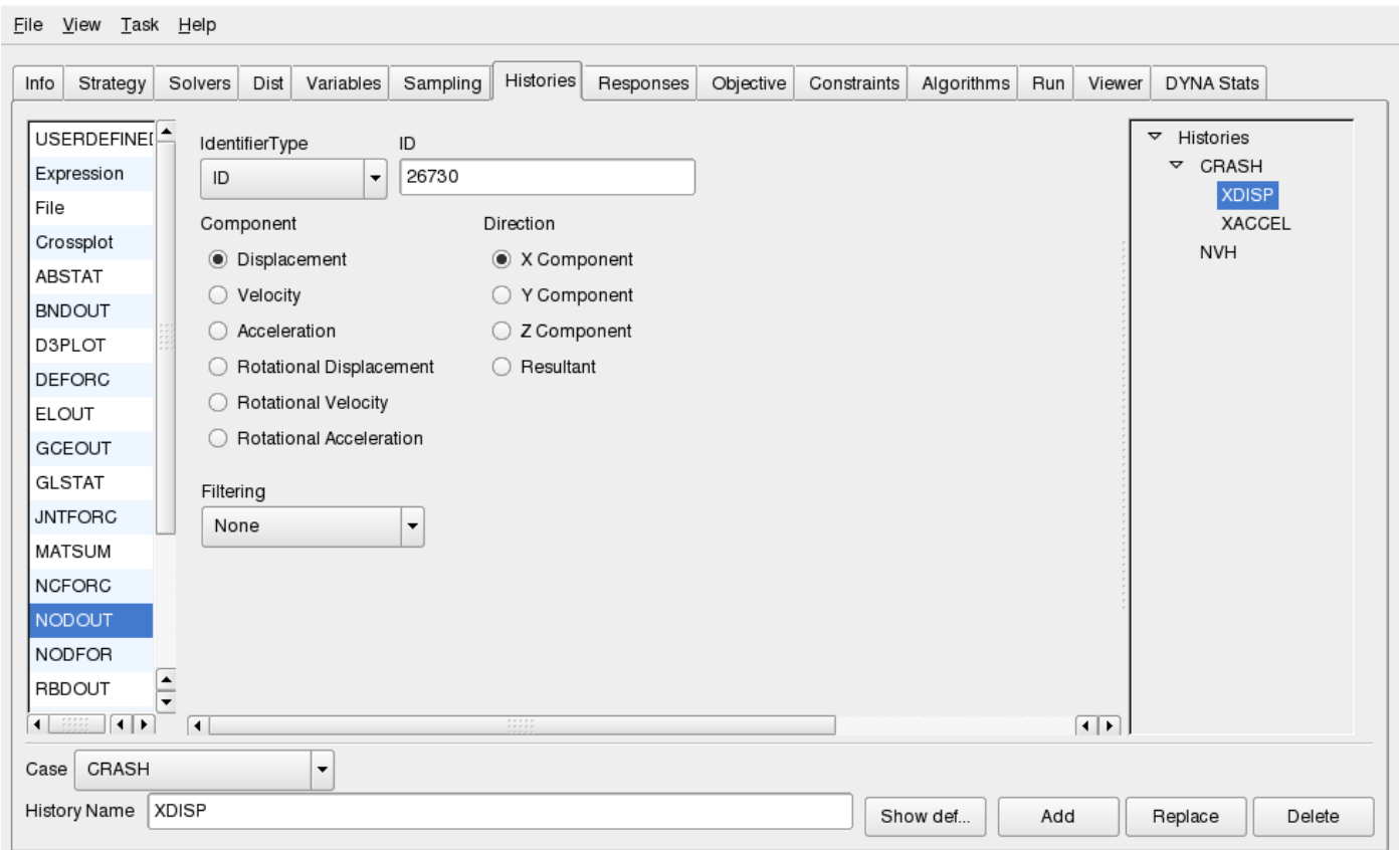
Figure 14-1: Histories panel in LS-OPT ui
