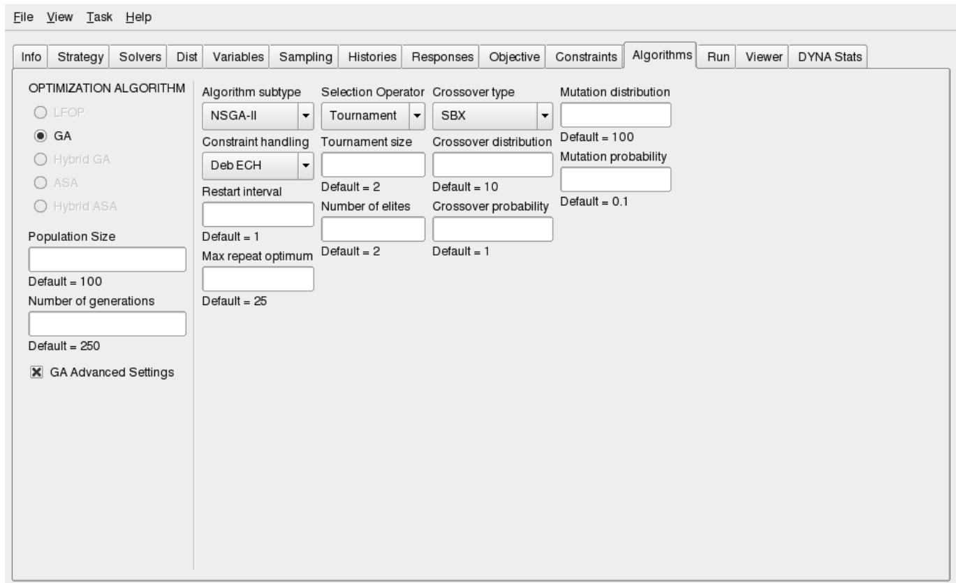
Figure 20-7: Selection of the GA parameters for creating a Pareto Optimal Frontier
