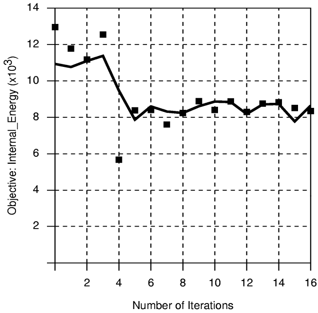
c) Internal_Energy
