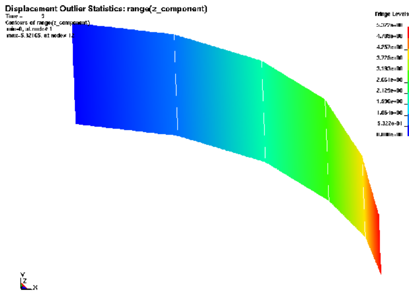
Figure 22-46 Second buckling mode
