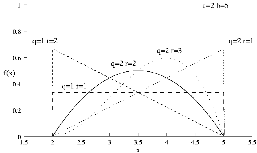
Figure 12-1 Beta distribution
