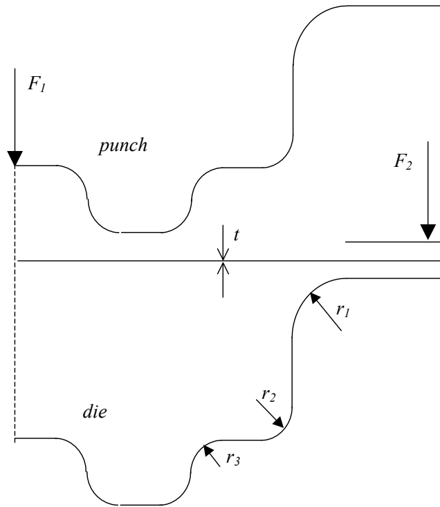
Figure 22-22: Parameterization of cross-section
