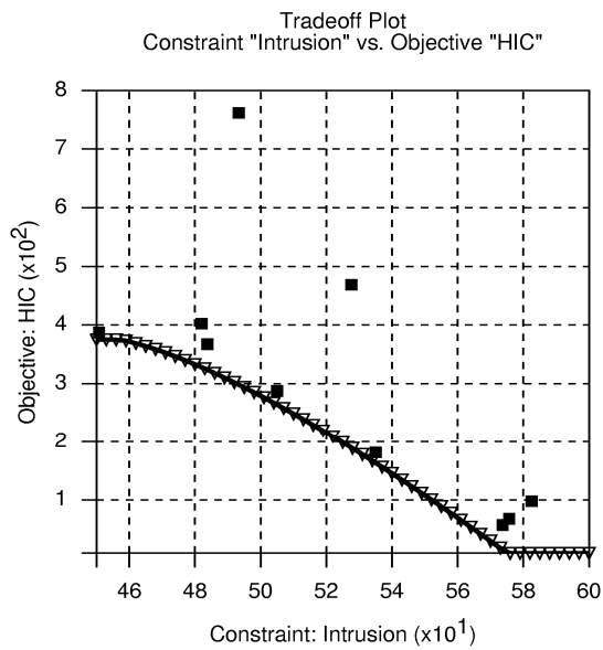
c) Trade-off of HIC versus Intrusion
