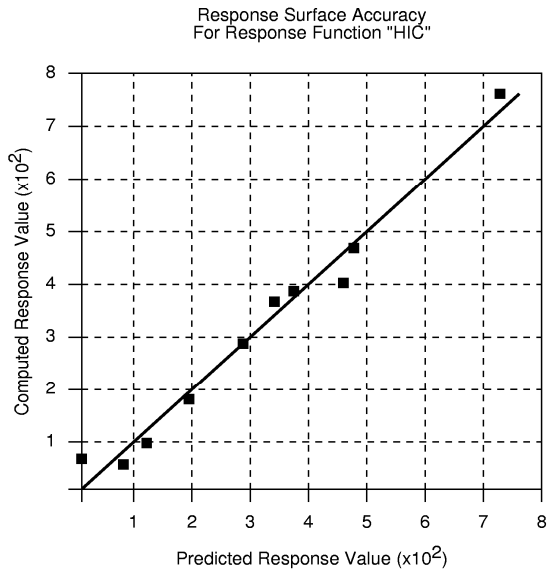
a) HIC response
