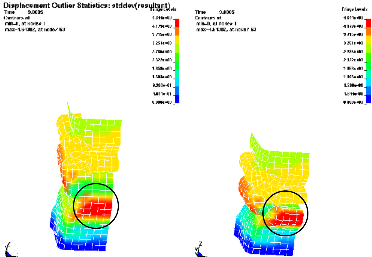
Figure 22-47 Tube Buckling
