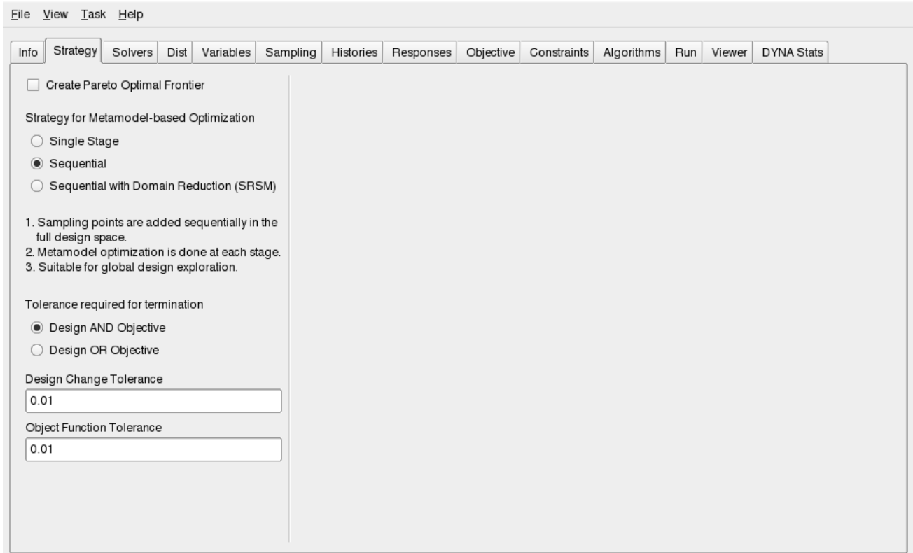
Figure 20-3: Sequential strategy selected in Strategy tab
