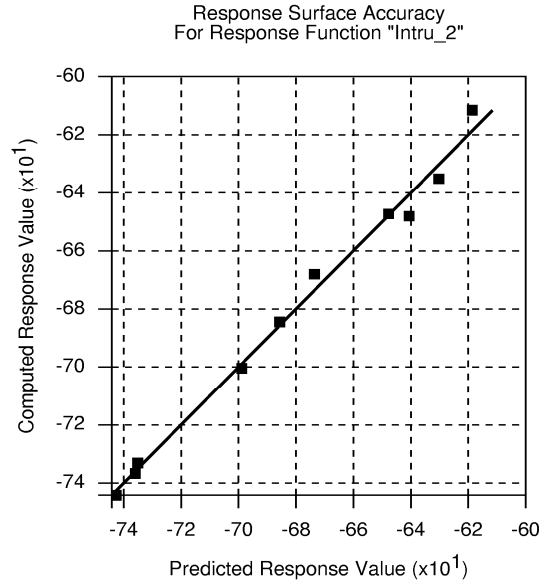
b) Intru_2 response
