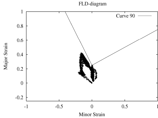
FLD diagram of 10 th iteration
