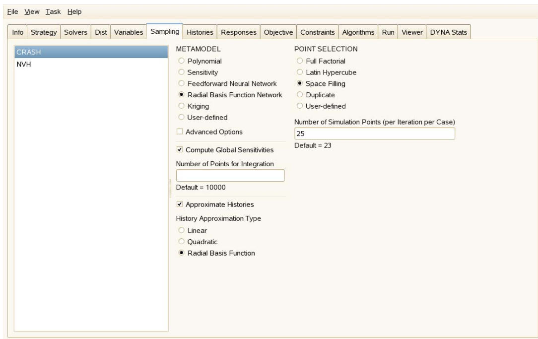
Figure 13-1: Sampling panel in LS-OPT
