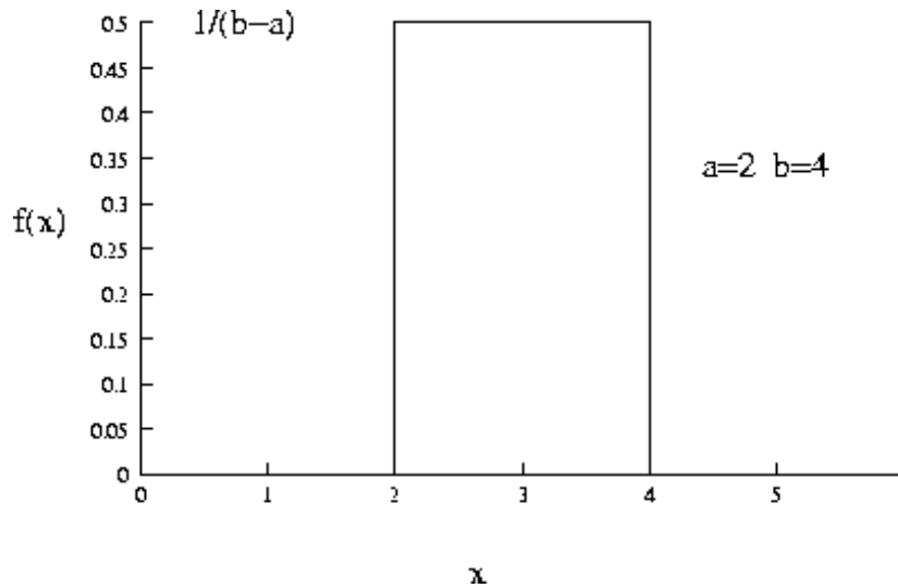
Figure 12-6 Uniform Distribution
