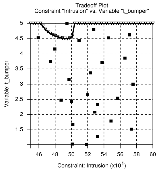
b) t_{bumper} versus Intrusion constraint
