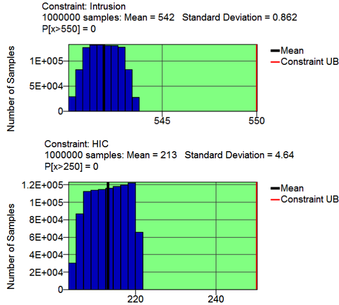
Figure 22-37: Frequency histogram of HIC and Intrusion with feasibility information. The green background shows that the designs are feasible within the tolerance interval.
