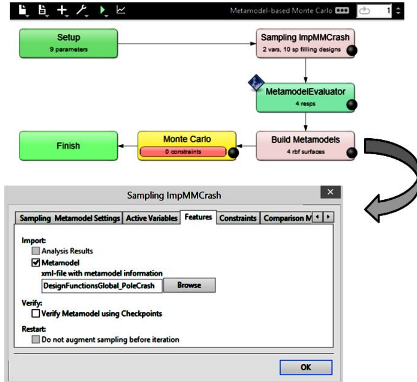
Figure 22-32: Monte Carlo analysis using imported metamodels
