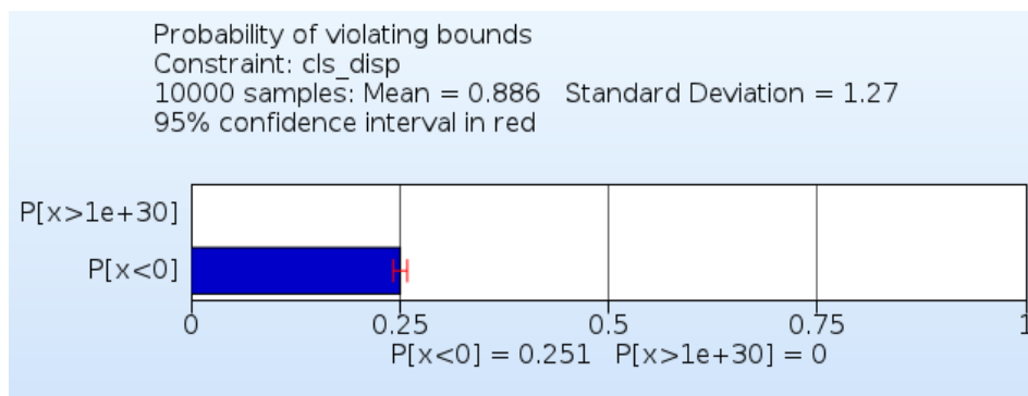
Figure 22-12: Classifier-based failure probability
