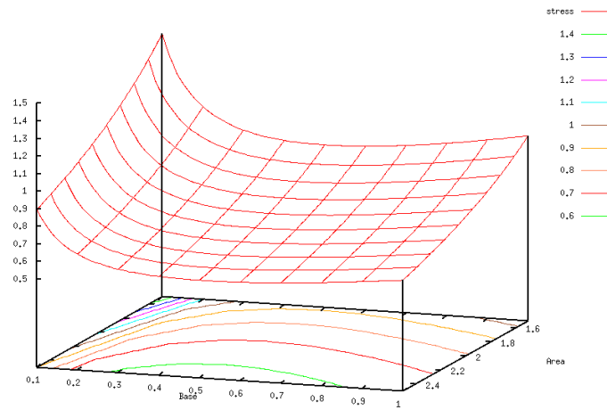
Figure 22-29: Contours of stress response. The flattest part of the response is when variable 'base' = 0.5.
