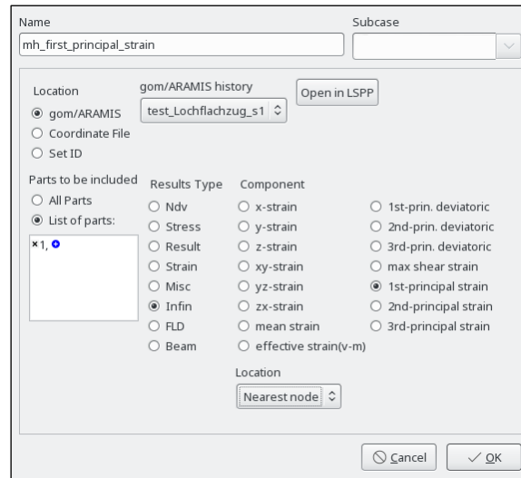
Figure 28-10: Multi-point history interface enabling the definition of the response type and location data. Location type can be defined as 'nearest node' or 'element'. In the latter option, the result is interpolated at the precise location within the nearest element.
