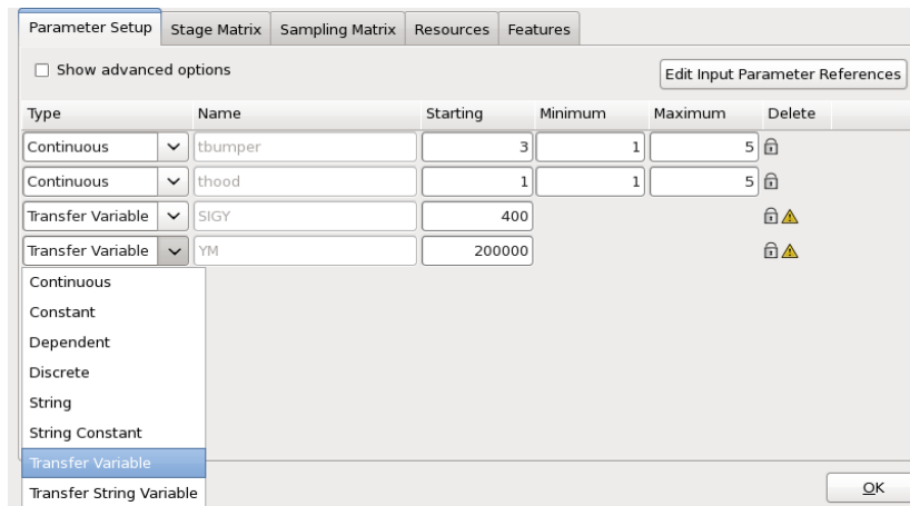
Figure 5-9: Parameterization of inner level LS-OPT setup using Transfer Variables. The values of transfer variables are passed down from the upper level(s).
