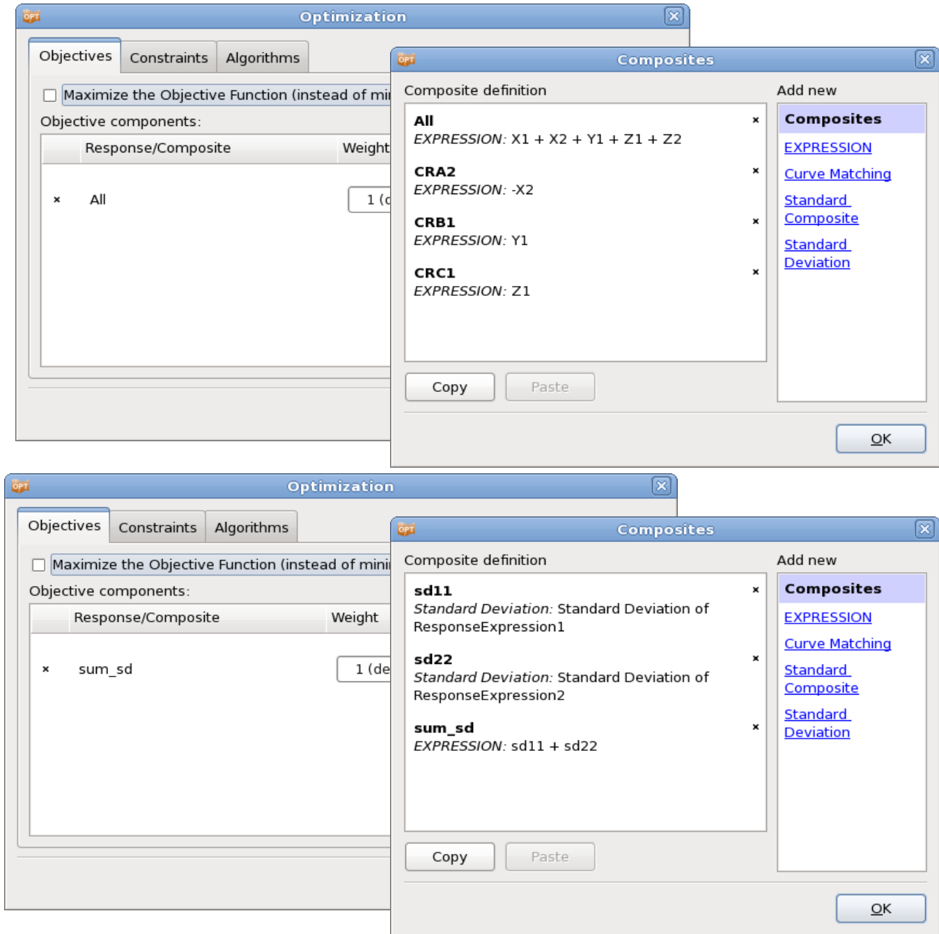
Figure 14-16: An example of objective function for RBDO (top) and robust design (bottom). Standard deviation is defined as the objective in latter case.
