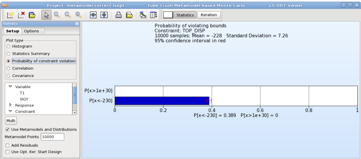
Figure 16-52: Probability of Response TOP_DISP < -230 with 95% confidence interval in red constructed using metamodel together with the statistical distribution of the variables
