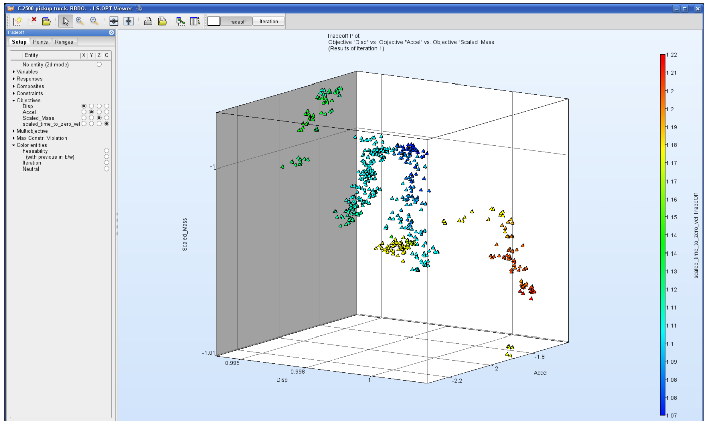
Figure 16-45: Tradeoff plot
