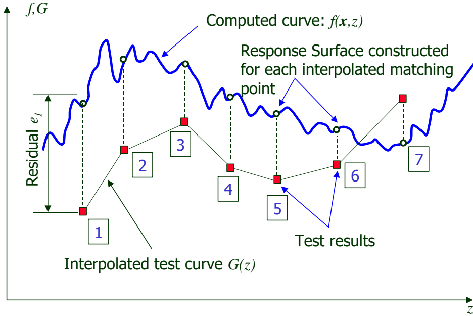
Figure 28-1: Entities in Mean Squared Error formulation
