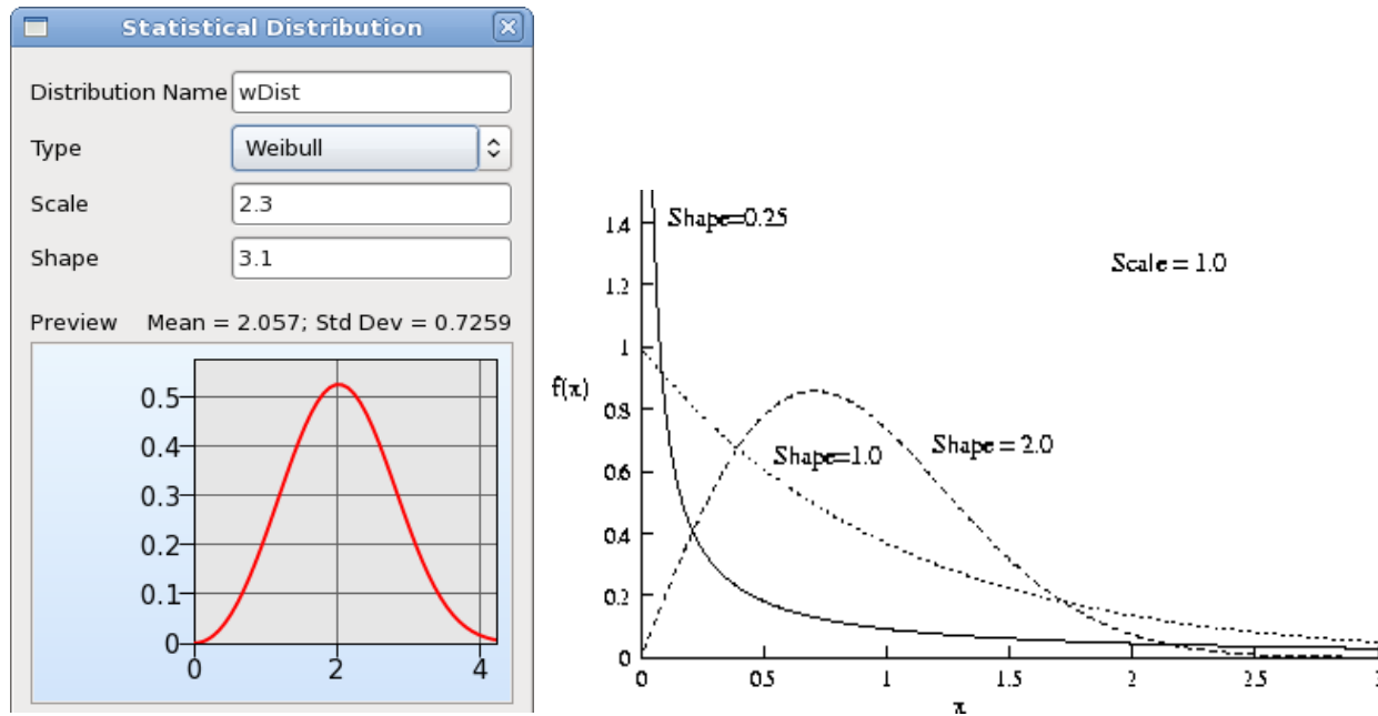
Figure 14-11: Weibull distribution
