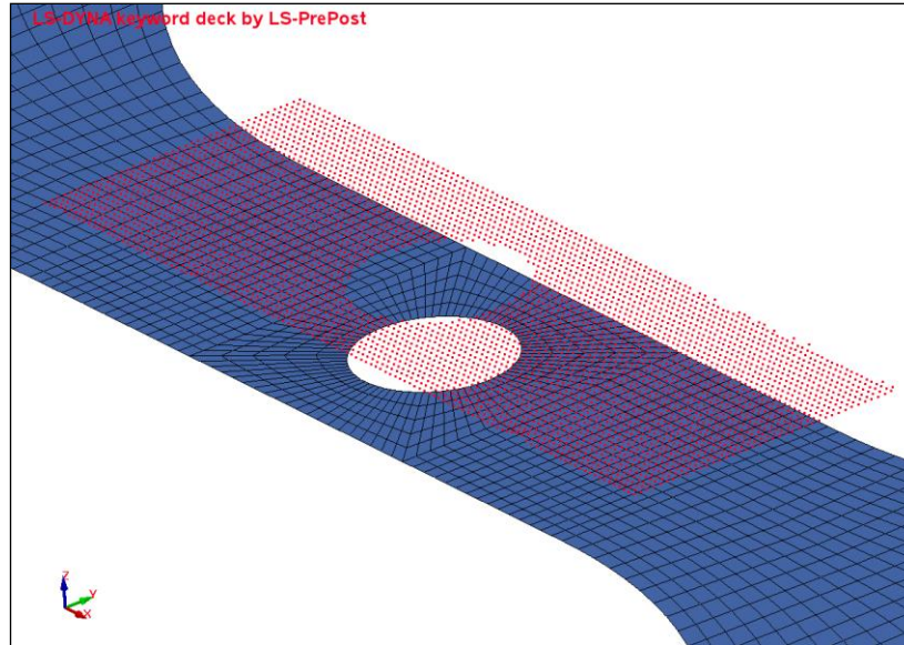
Figure 28-12: Example of test point mapping showing test point set (red) of 4557 points in relation to the Finite Element mesh.
