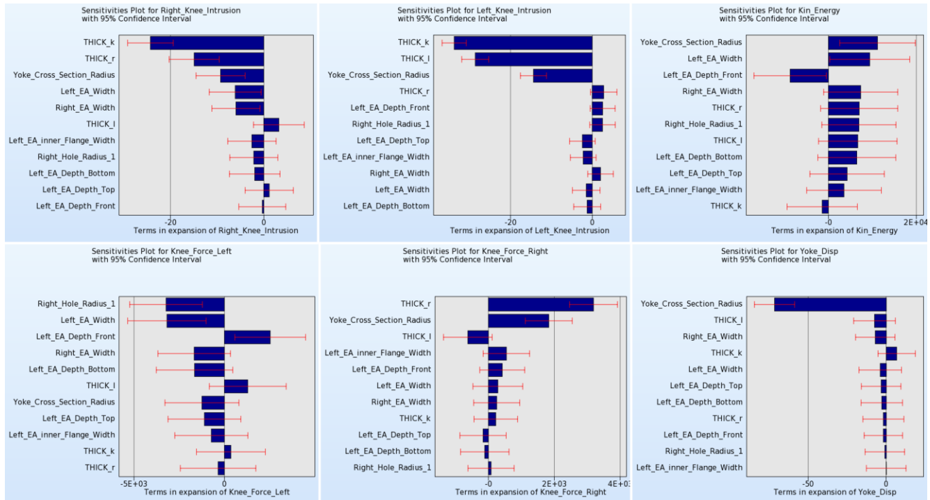
Figure 20-104: ANOVA plots for objectives and constraints of knee-bolster design problem.
