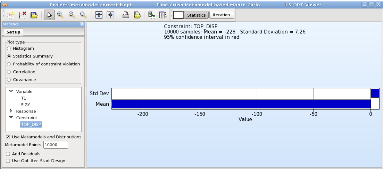
Figure 16-51: Mean value and standard deviation constructed using metamodel together with the statistical distribution of the variables
