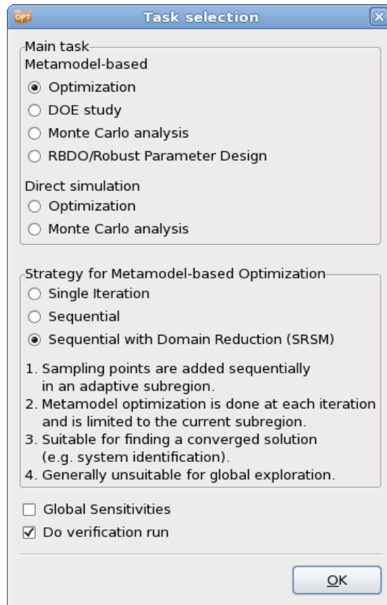
Figure 20-20: Task dialog; select strategy SRSM to automate the process.
