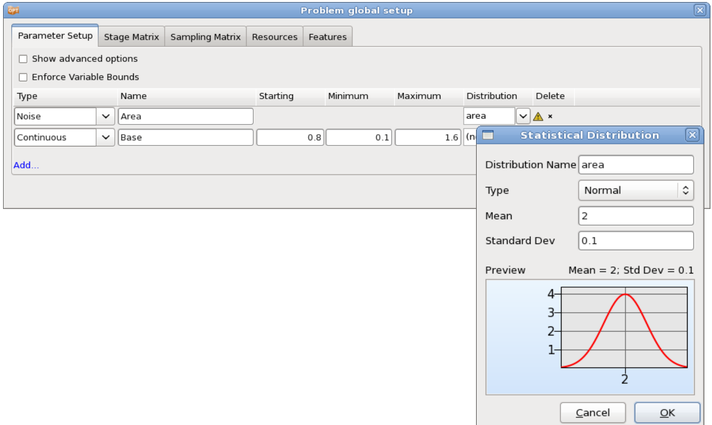
Figure 22-27: Parameter Setup and distribution
