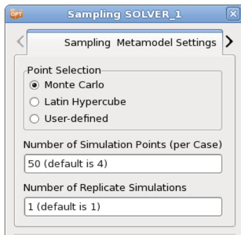
Figure 22-54: Sampling dialog. Specify the number of simulation points. The point selection doesn't affect the analysis here, since the variable is not used.
