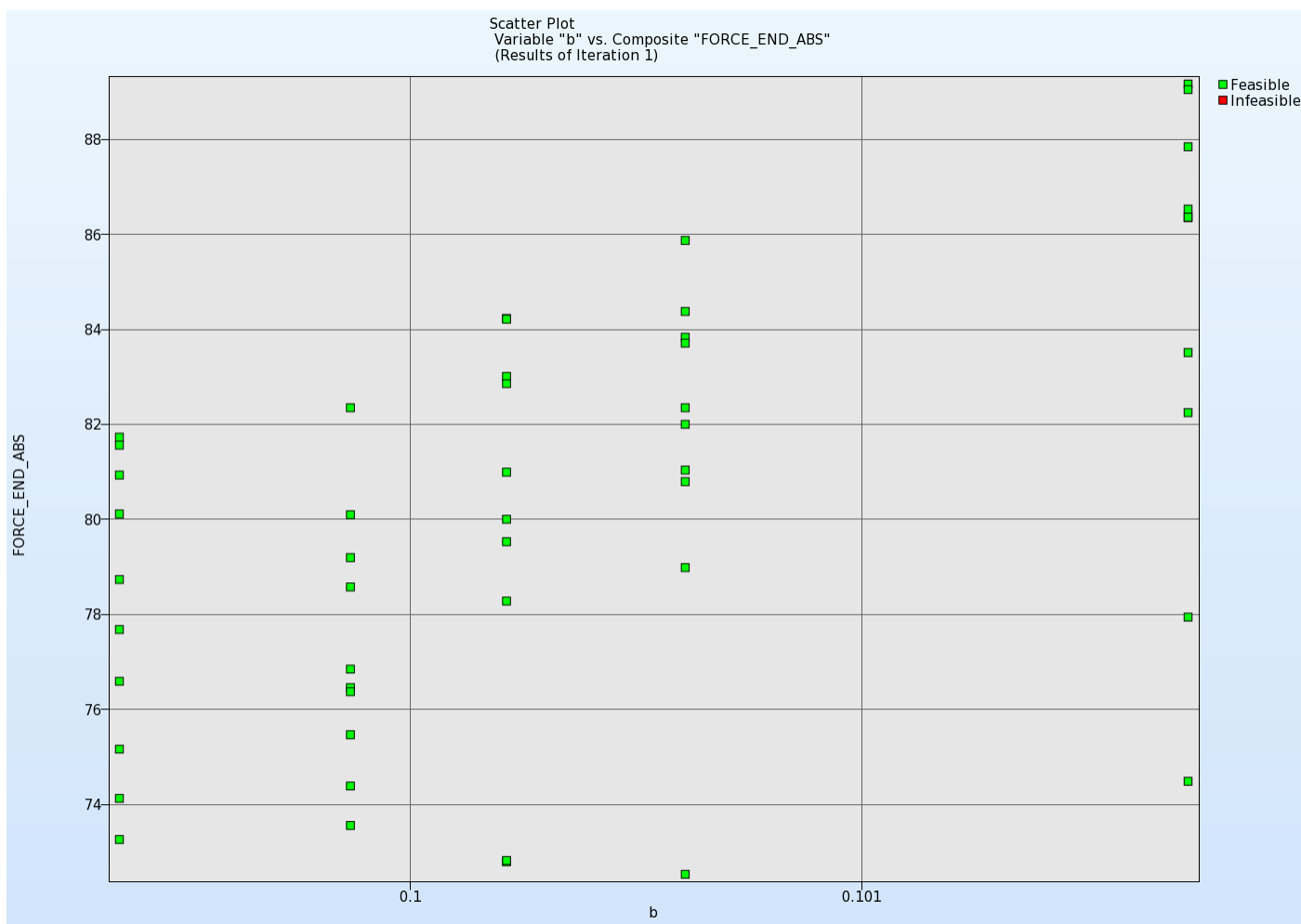
Figure 22-60: Plot of the responses using replicate experiments
