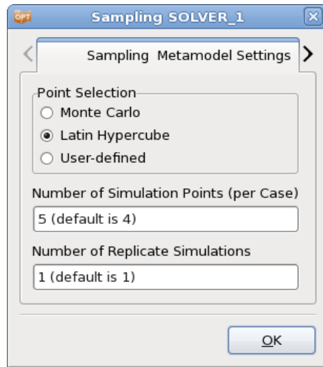
Figure 22-16: Definition of Latin Hypercube sampling with 5 points.
