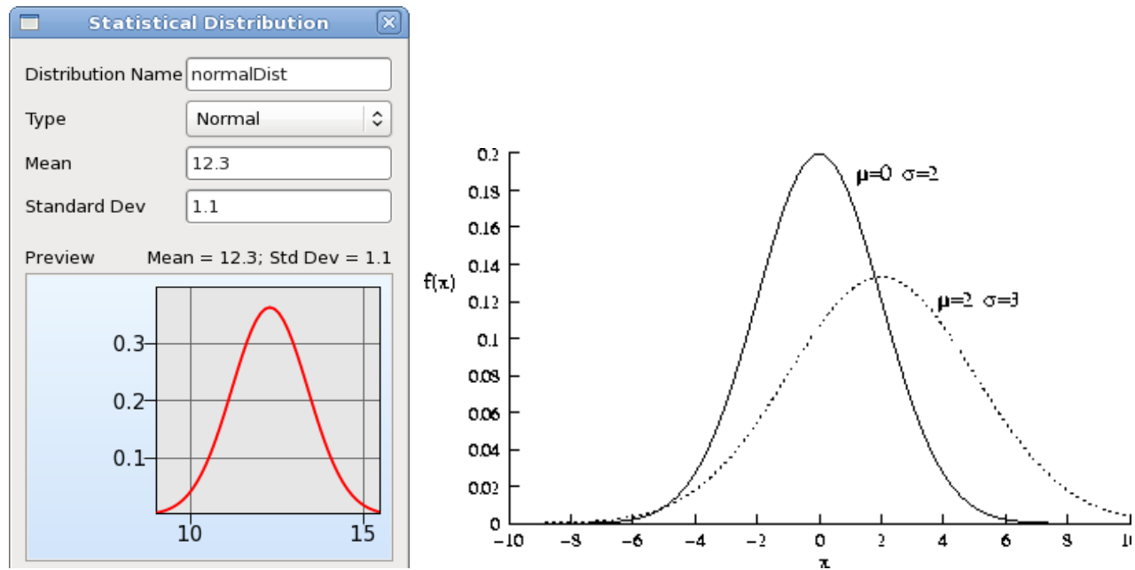
Figure 14-5: Normal Distribution
