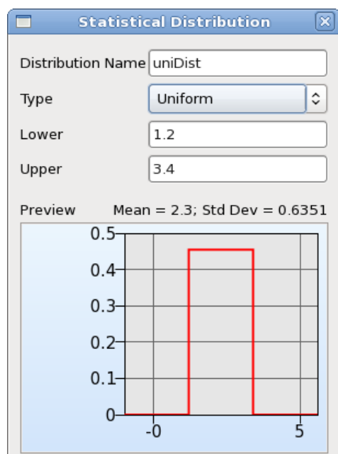
Figure 14-7: Uniform Distribution
