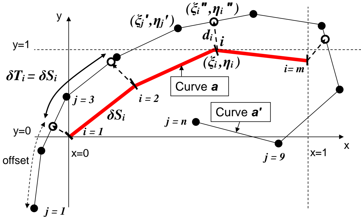
Figure 28-6: Partial curve mapping of Curve a (in red) to Curve a' with offset. The result is Curve a'' . The solid points represent the original vertices of a' whereas the open circles represent the mapped points representing a'' . Curves a and a' are both normalized to the bounding box of a .
