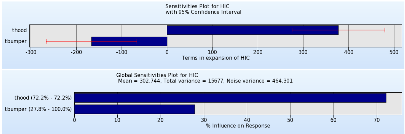
Figure 20-31: Sensitivity plots; ANOVA with 95% confidence interval (top) and GSA (bottom)
