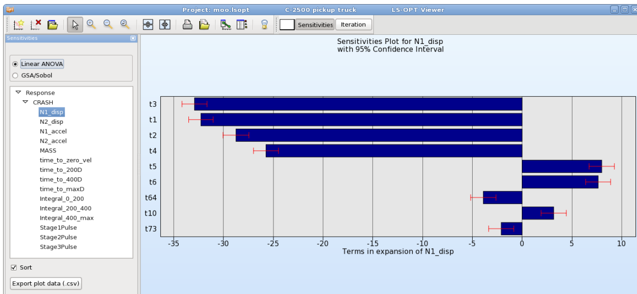
Figure 16-38: Linear ANOVA plot, sorted
