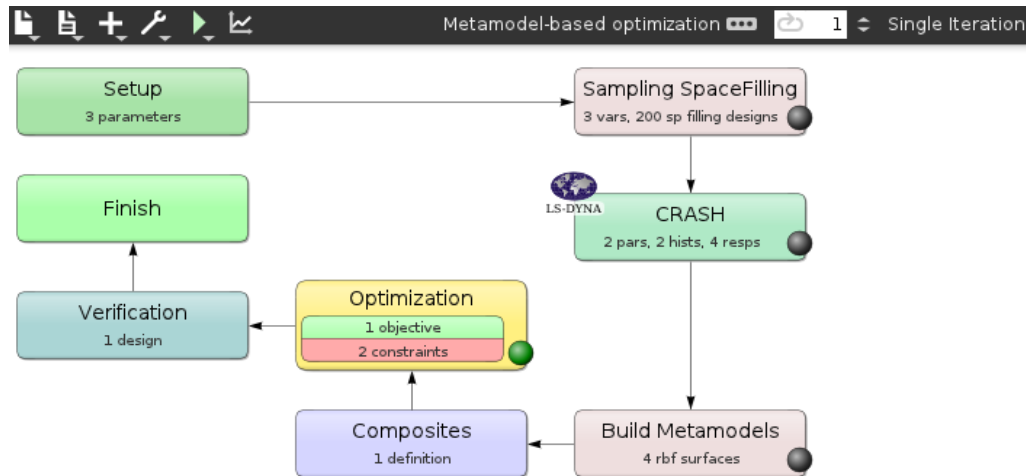
Figure 22-39: LS-OPT setup for Step 1 (global approximation and deterministic optimization)
