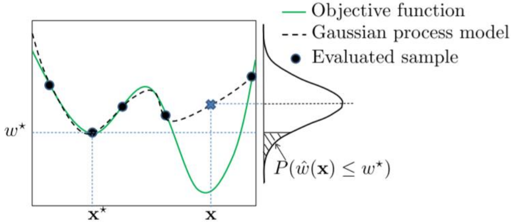
Figure 26-3: Probability of improvement at a design configuration based on Kriging. This point has a higher mean objective function prediction than the current best \mathbf{x}^* , but has a non-zero probability of improvement due to higher variance. The variance at evaluated samples is zero.
