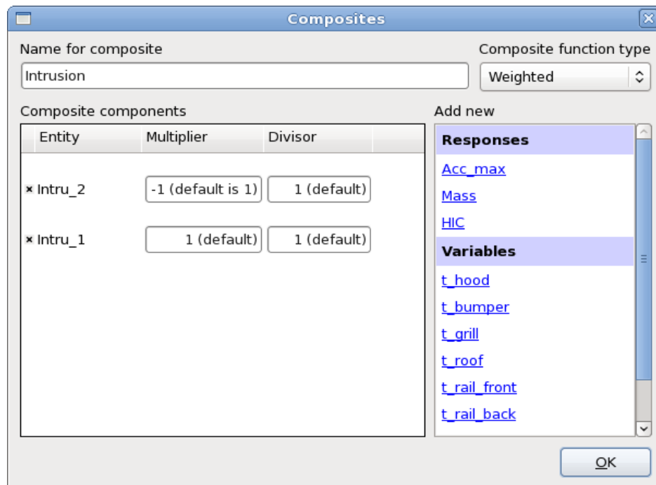
Figure 10-3: Standard Composite Interface
