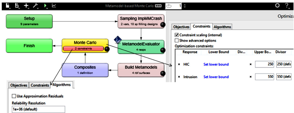
Figure 22-35: Monte Carlo analysis setup. The number of Monte Carlo samples used for calculations based on the imported metamodel are defined as the Reliability Resolution.
