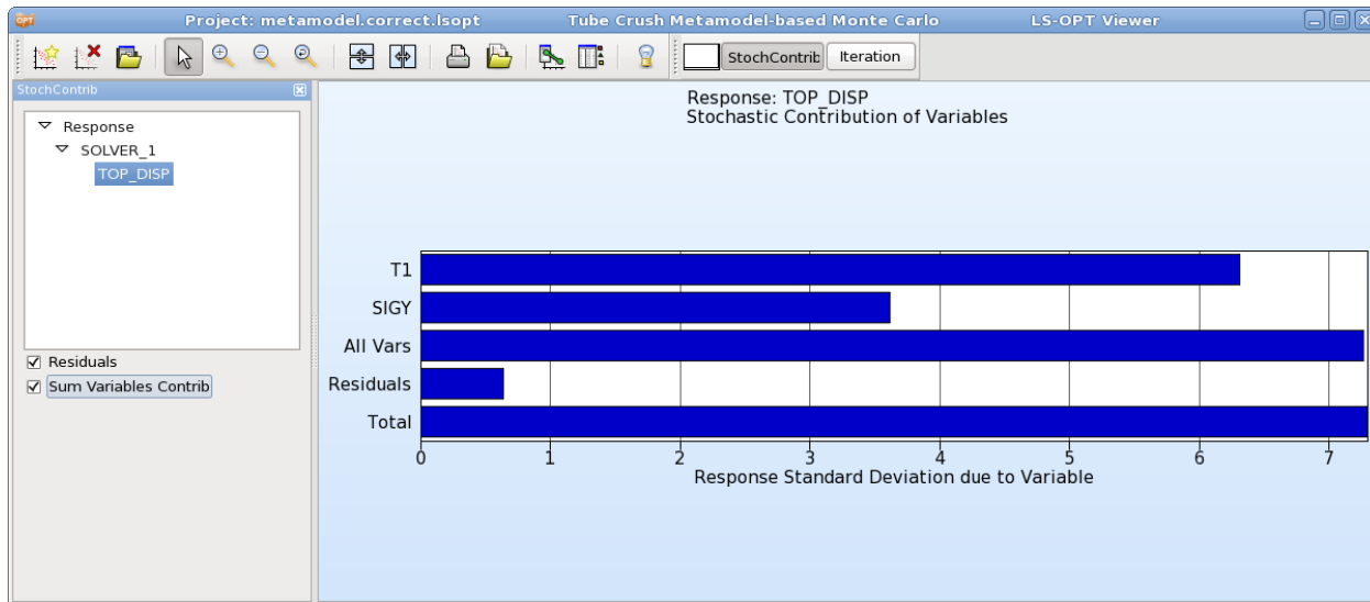
Figure 16-55: Stochastic Contribution plot
