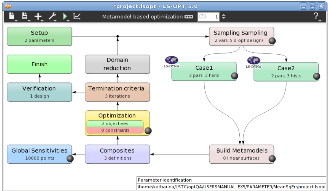
Figure 21-2: LS-OPT main GUI window
