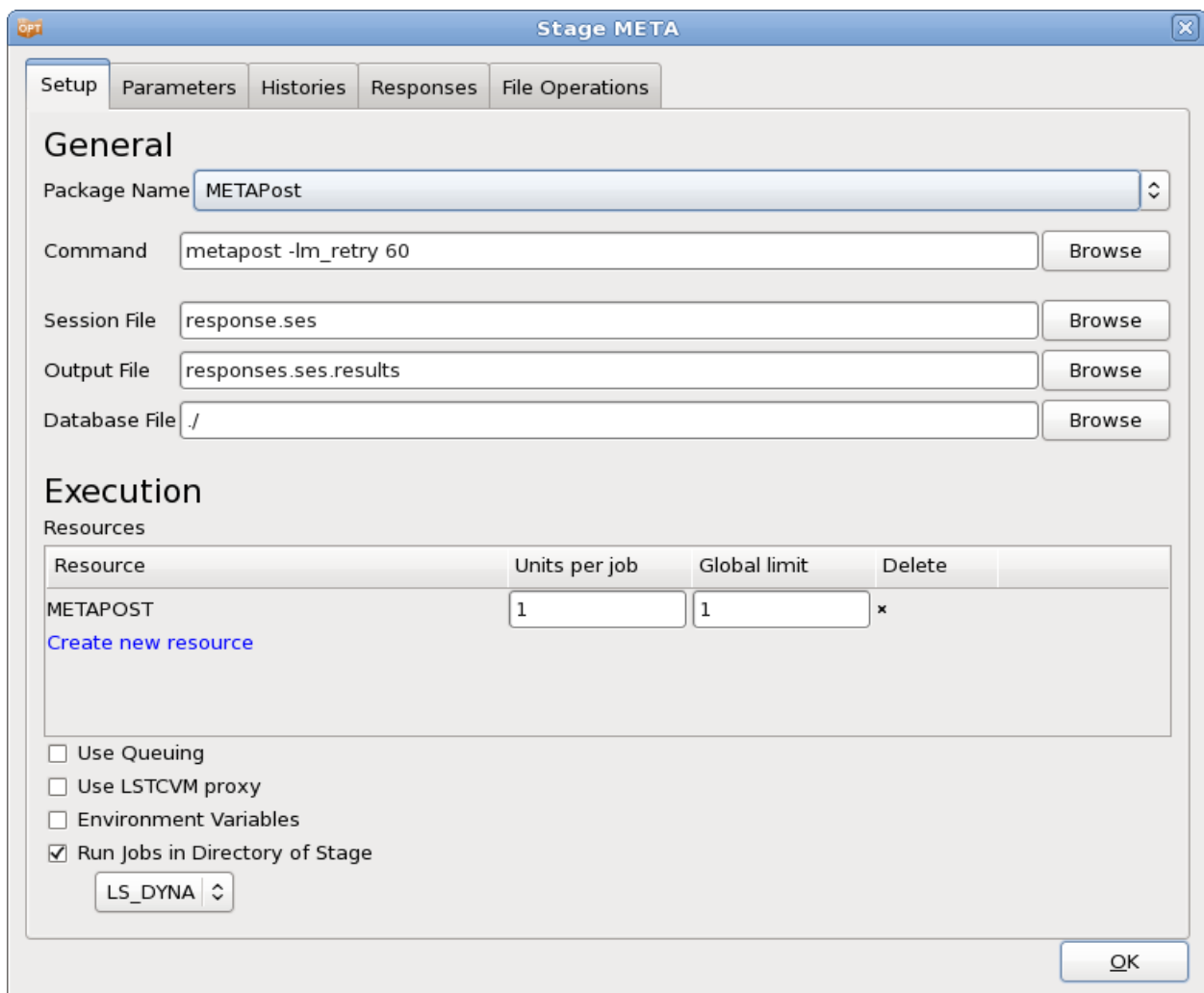
Figure 20-112: Stage dialog interfacing with \mu ETApост. \mu ETApост is run in the respective LS-DYNA run directory, since the results are extracted from the LS-DYNA output.
