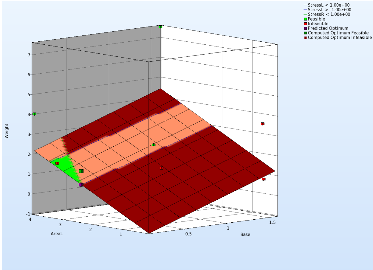
Figure 20-11: Surface plot for objective function Weight; constraints are displayed on the metamodel.
