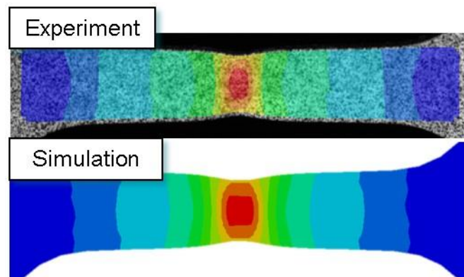
Figure 28-8: Full field measurement of a tensile test using Digital Image Correlation. Above is the DIC image (GOM ARAMIS) while a strain contour plot is featured below (LS-PrePost®).
