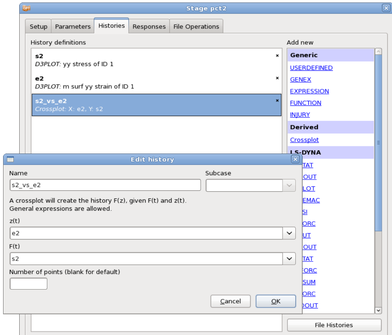
Figure 21-17: History definitions. Extract stress and strain using the LS-DYNA d3plot interface. Use the Crossplot interface to generate the stress vs. strain curve
