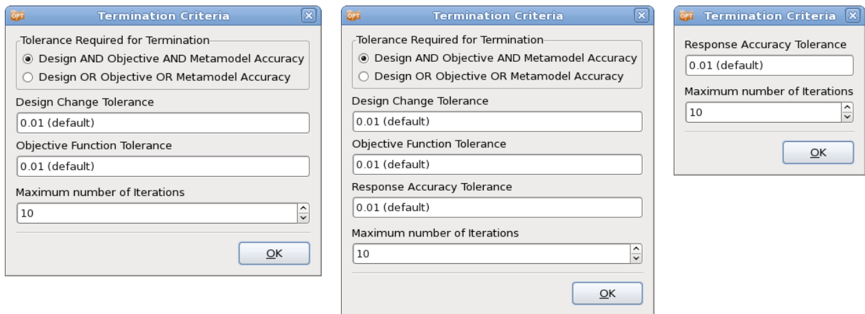
Figure 13-1: Termination Criteria dialog for metamodel based optimization using different methods – single objective sequential with domain reduction or efficient global optimization (left), single objective sequential (middle), multi-objective sequential.
