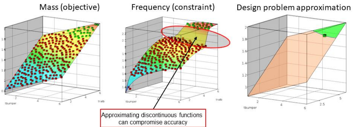
Figure 20-139: FNN approximation for mass minimization with torsional frequency constraint. The frequency response is discontinuous due to mode switching.
