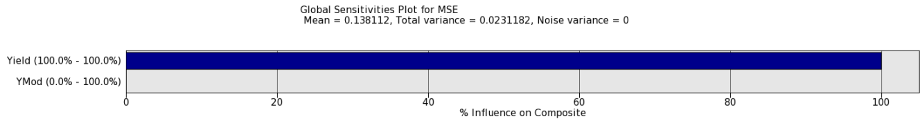
Figure 19-2: Global Sensitivities
