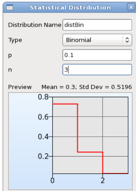
Figure 14-3: Binomial distribution
