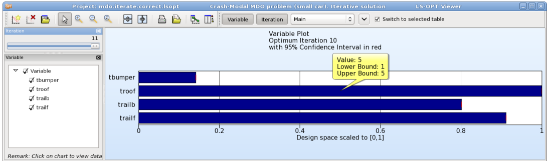
Figure 16-44: Variable Plot
