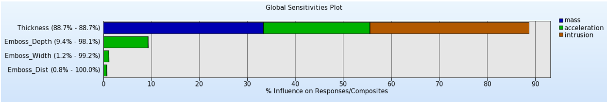
Figure 20-115: Global Sensitivities.
