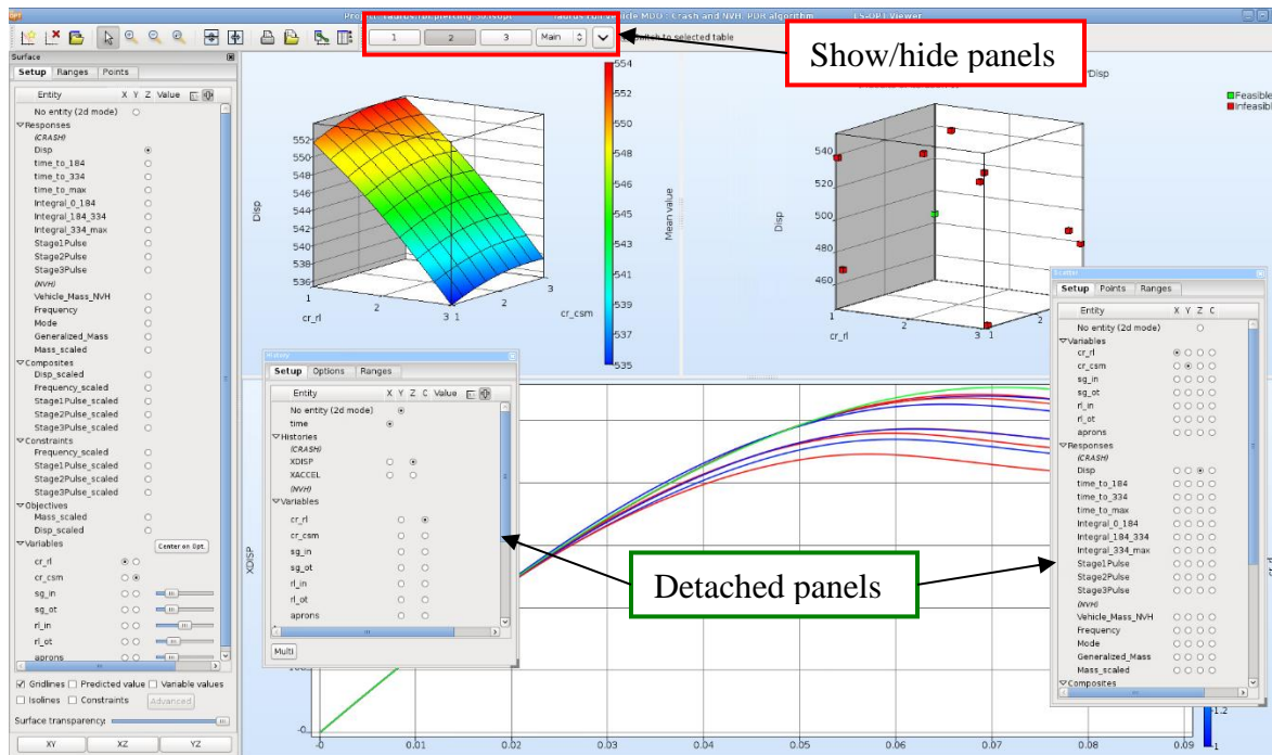
Figure 16-9: Detachable panels
