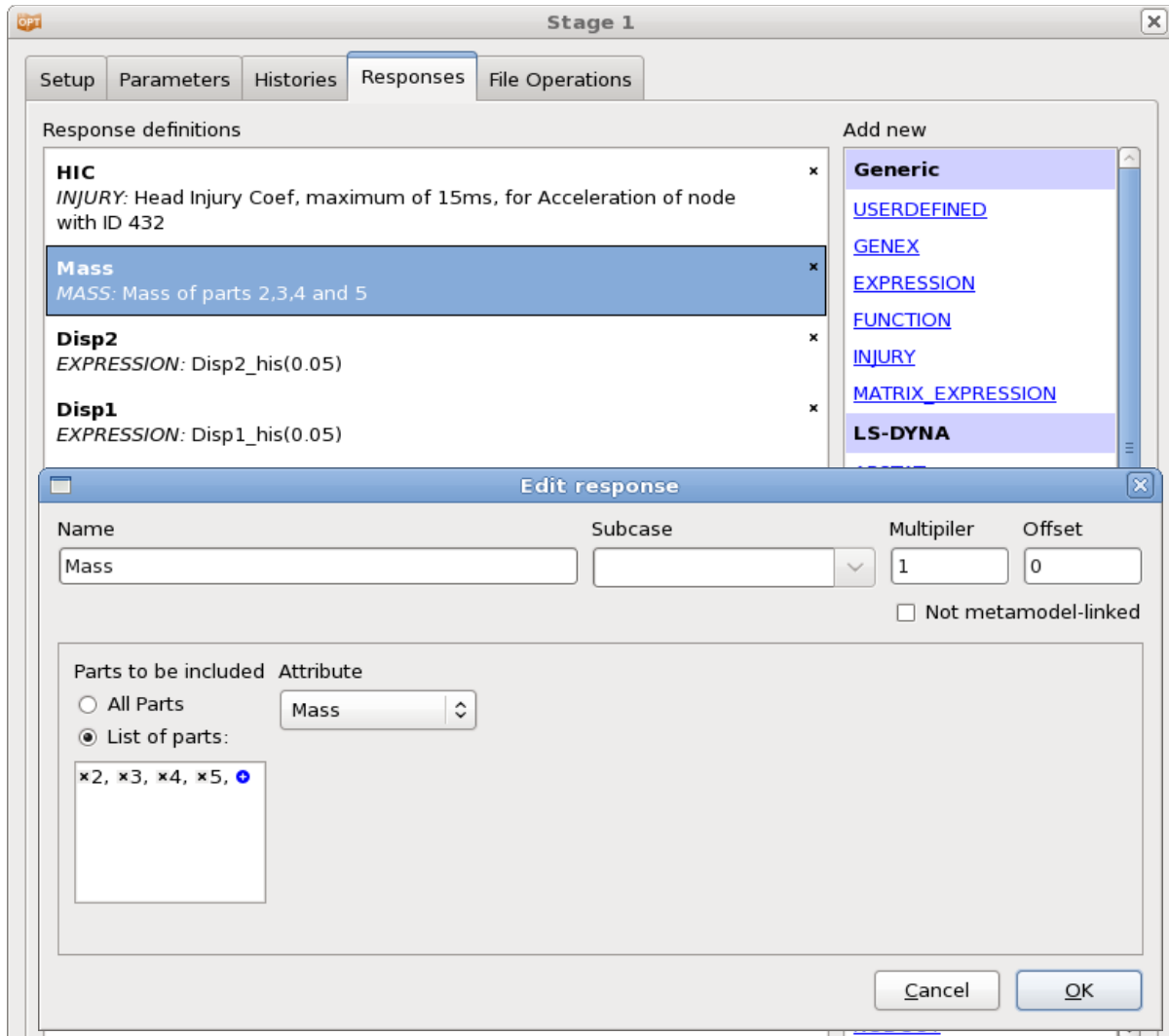
Figure 20-26: Definition of responses using standard LS-DYNA interfaces and expressions.
