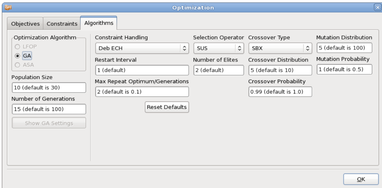
Figure 20-43: Optimization dialog; Specification of advanced GA options
