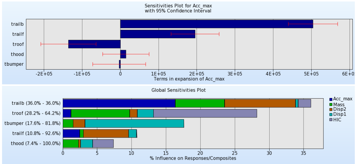
Figure 19-6: ANOVA values for a single response; Sobol values for multiple responses
