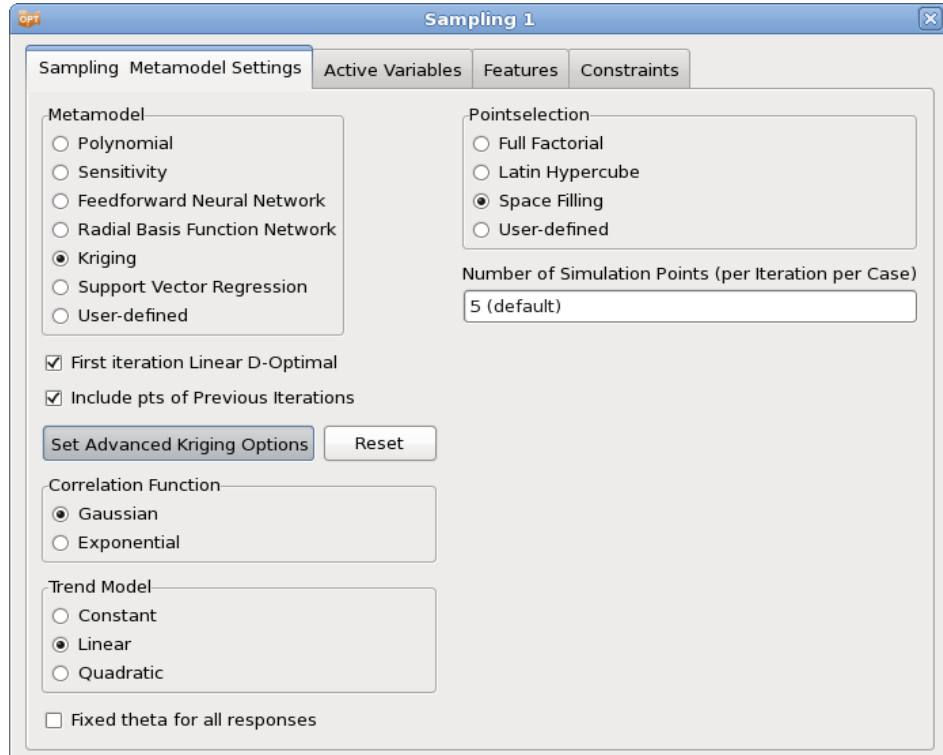
Figure 9-7: Kriging Advanced Options
