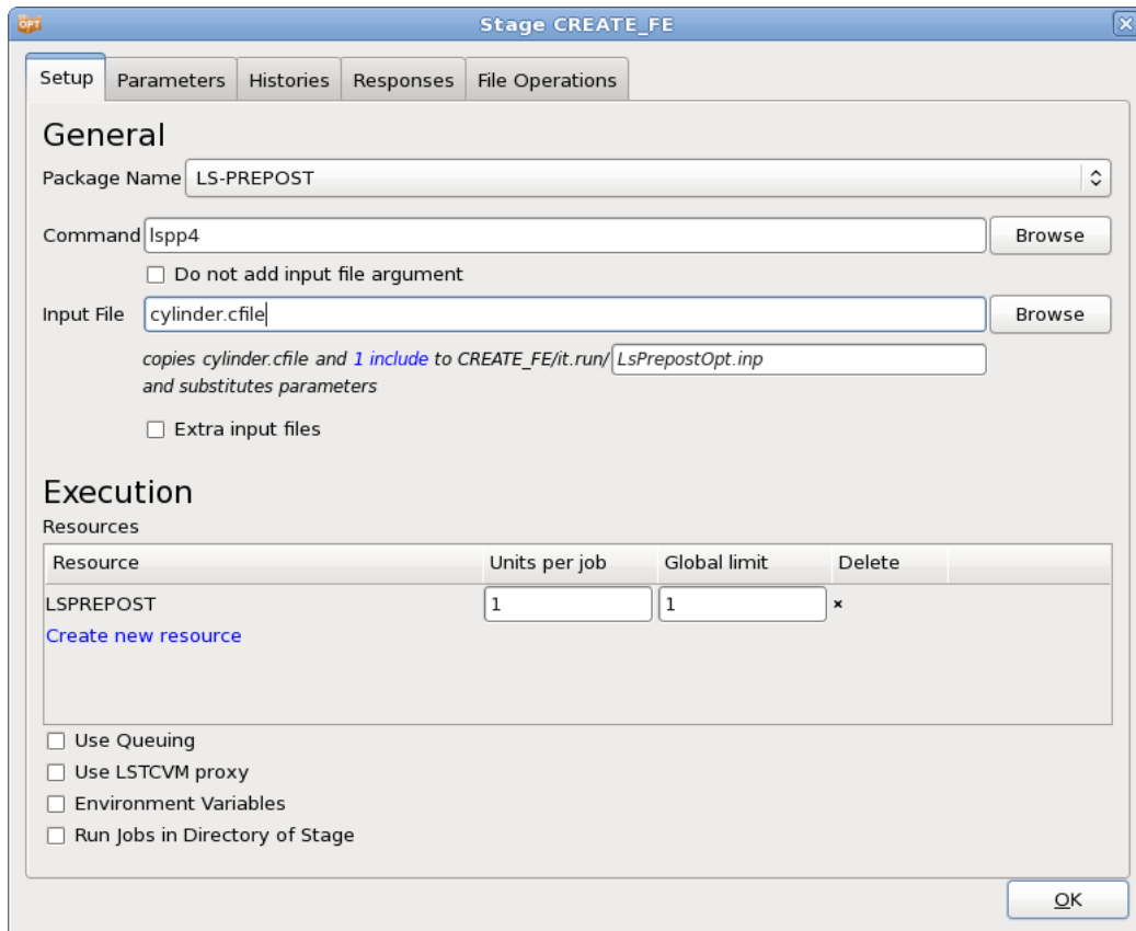
Figure 20-58: Stage dialog interfacing with LS-PREPOST
