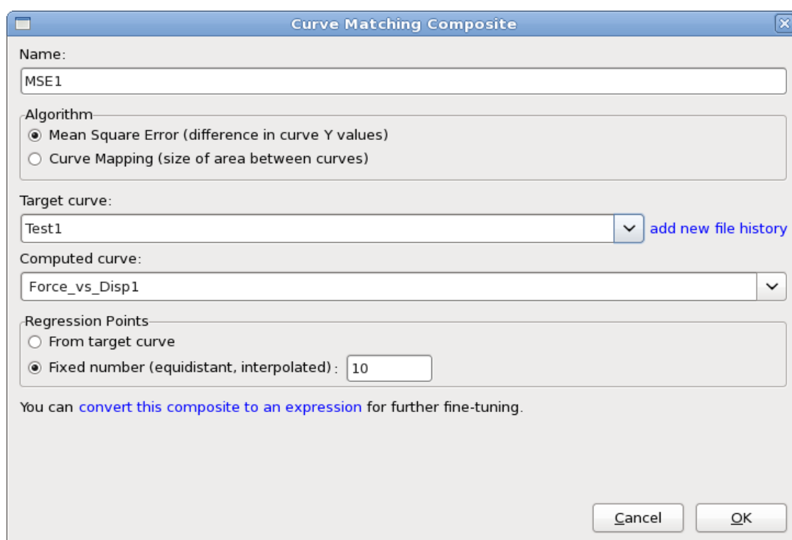
Figure 21-5: Definition of Mean Square Error composite
