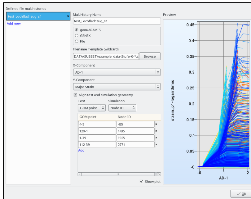
Figure 28-9: GOM ARAMIS interface in LS-OPT showing alignment input and verification plot of selected test value X- and Y-components.
