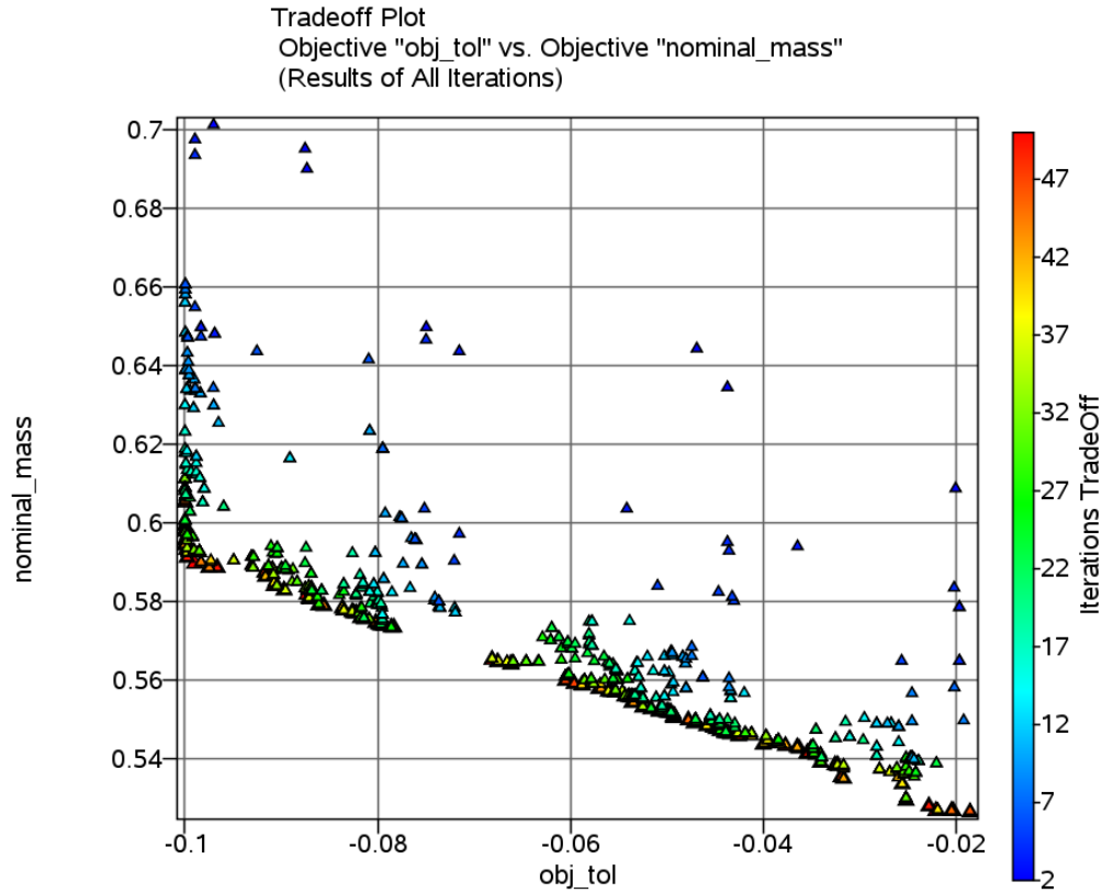
Figure 22-50: Tradeoff between mass and tolerance objectives for all iterations.
