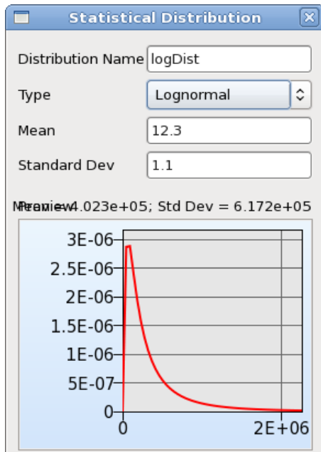
Figure 14-4: Lognormal distribution
