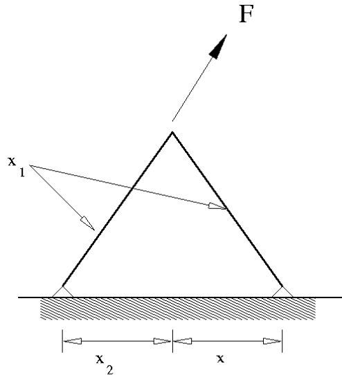
Figure 22-25: The two-bar truss problem. The problem has two variables: the thickness of the bars and the leg widths as shown. The bar thicknesses are noise variables while the leg widths are adjusted (control variables) to minimize the effect of the variation of the bar thicknesses. The maximum stress in the structure is monitored.
