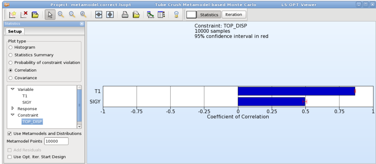
Figure 16-53: Correlation Bars evaluated on metamodel
