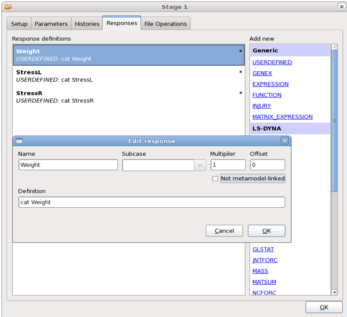
Figure 20-3: User-defined response definitions
