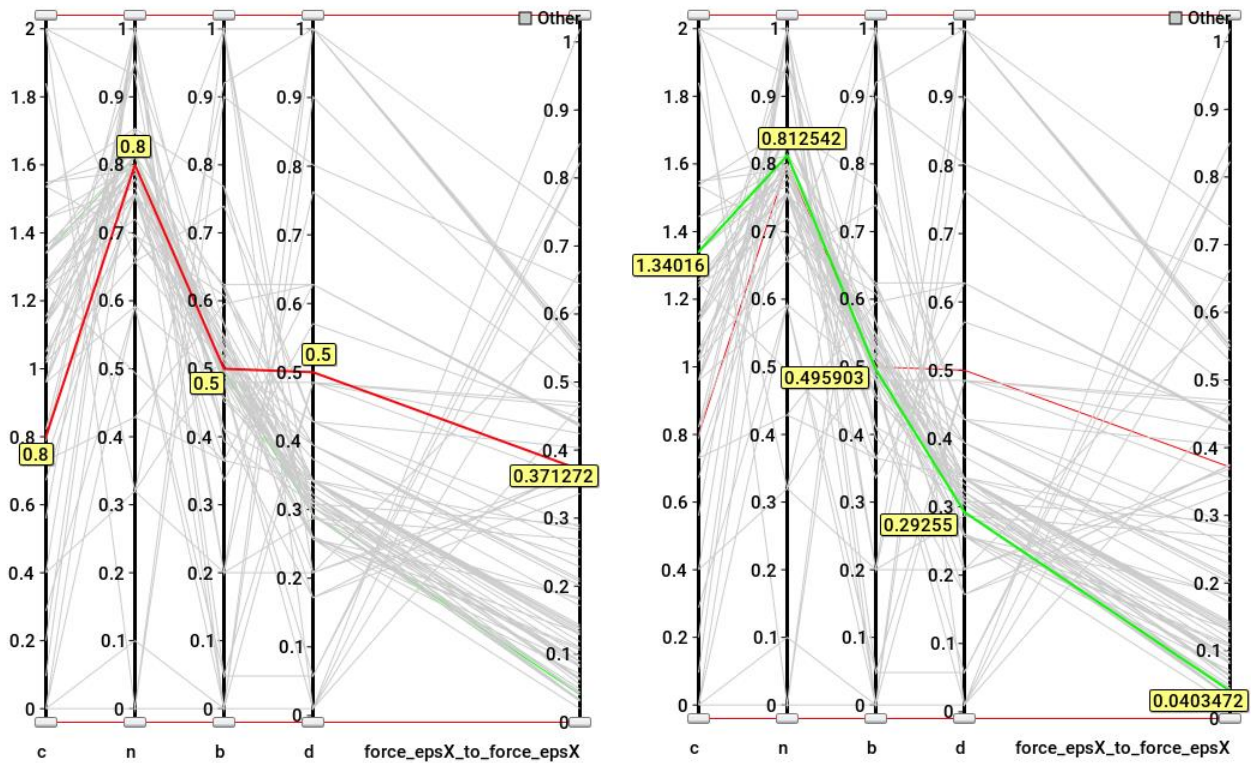
Figure 21-41: Baseline variables C , N , B and D together with objective value ( force_epsX_to_force_epsX ) in red (left) and optimum solution in green (right). The 'categories' option was used to highlight the relevant curve in red/green.
