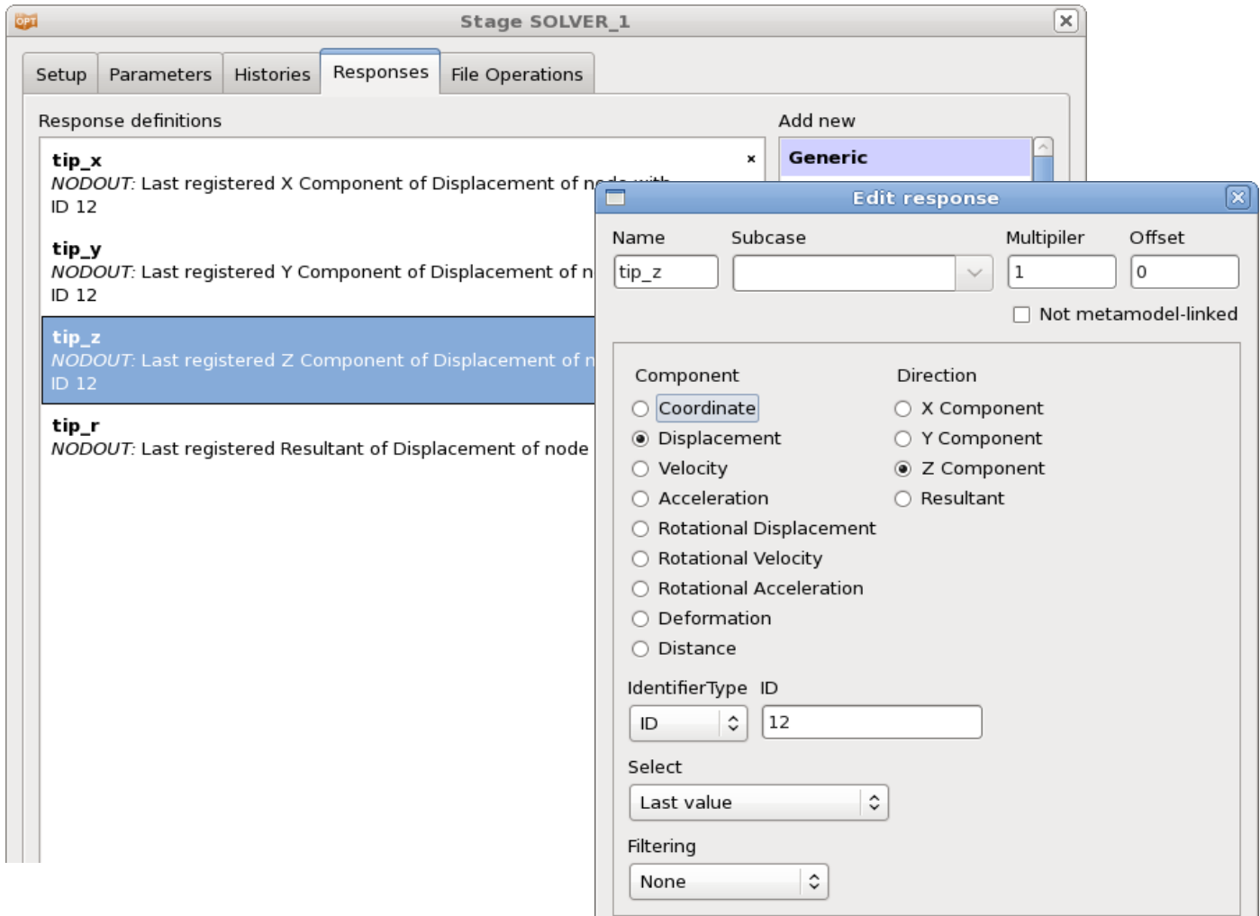
Figure 22-17: Response Definition for bifurcation identification
