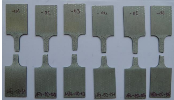
Figure 21-30: Test coupons for a tensile test ( 0^\circ w.r.t. rolling direction) 15
