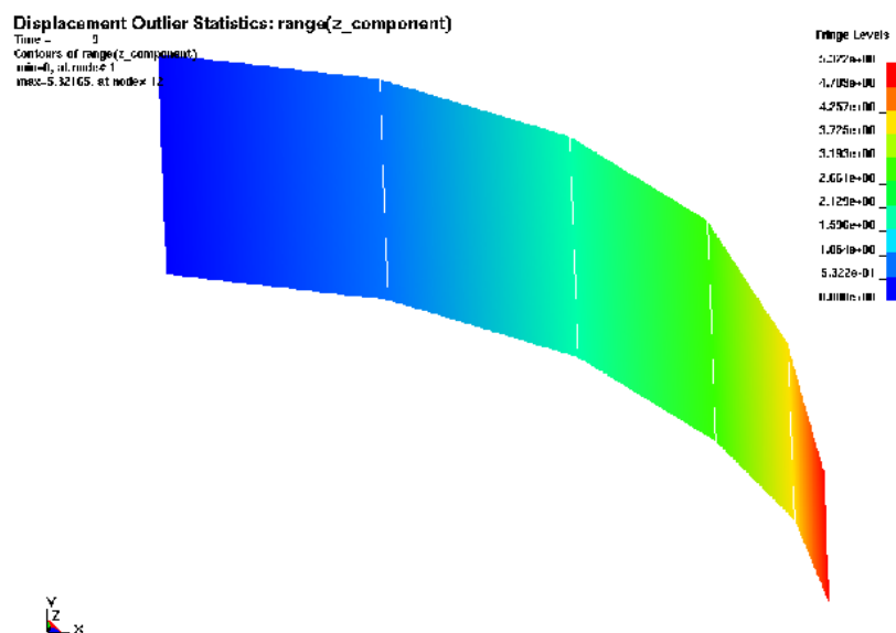
Figure 22-23: Second buckling mode
