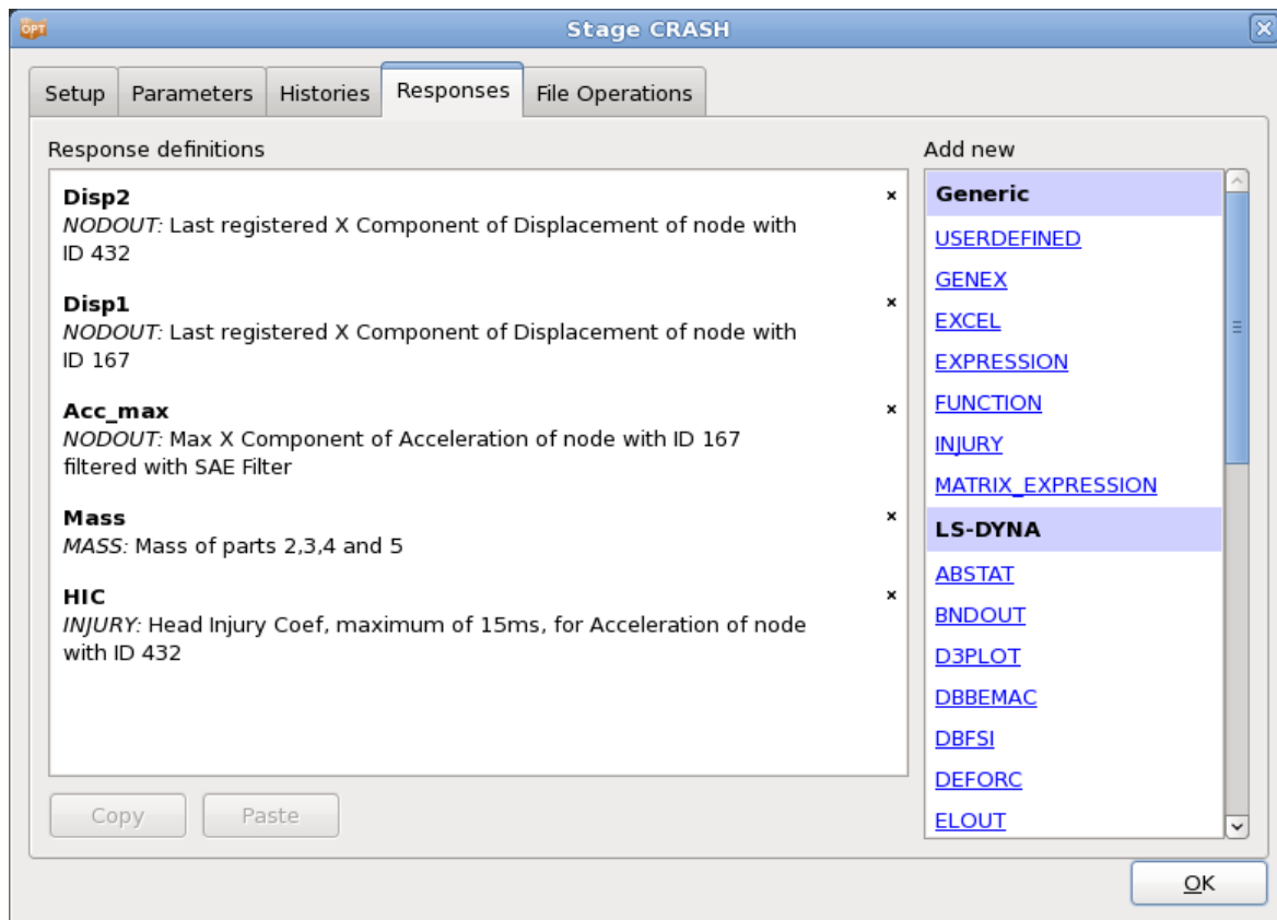
Figure 2-6: Stage dialog - Responses page. Select a response type from the list on the right to add a new response definition.
