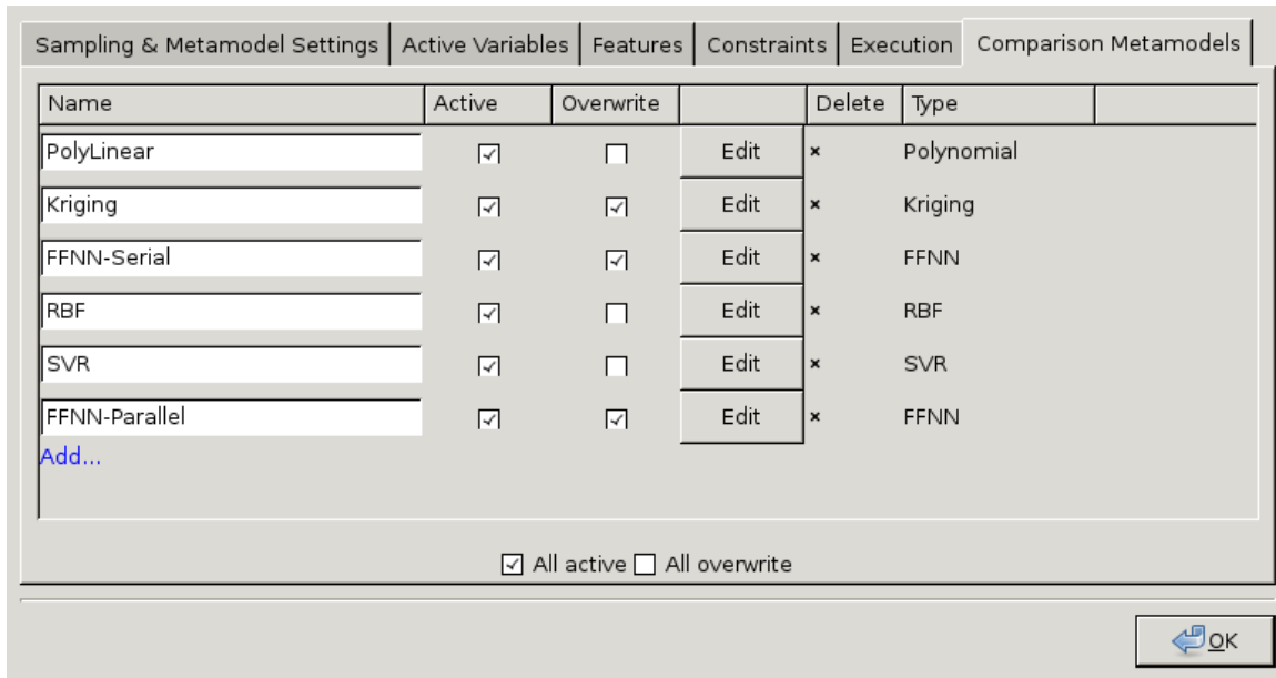
Figure 9-21: Definition of comparison metamodels.
