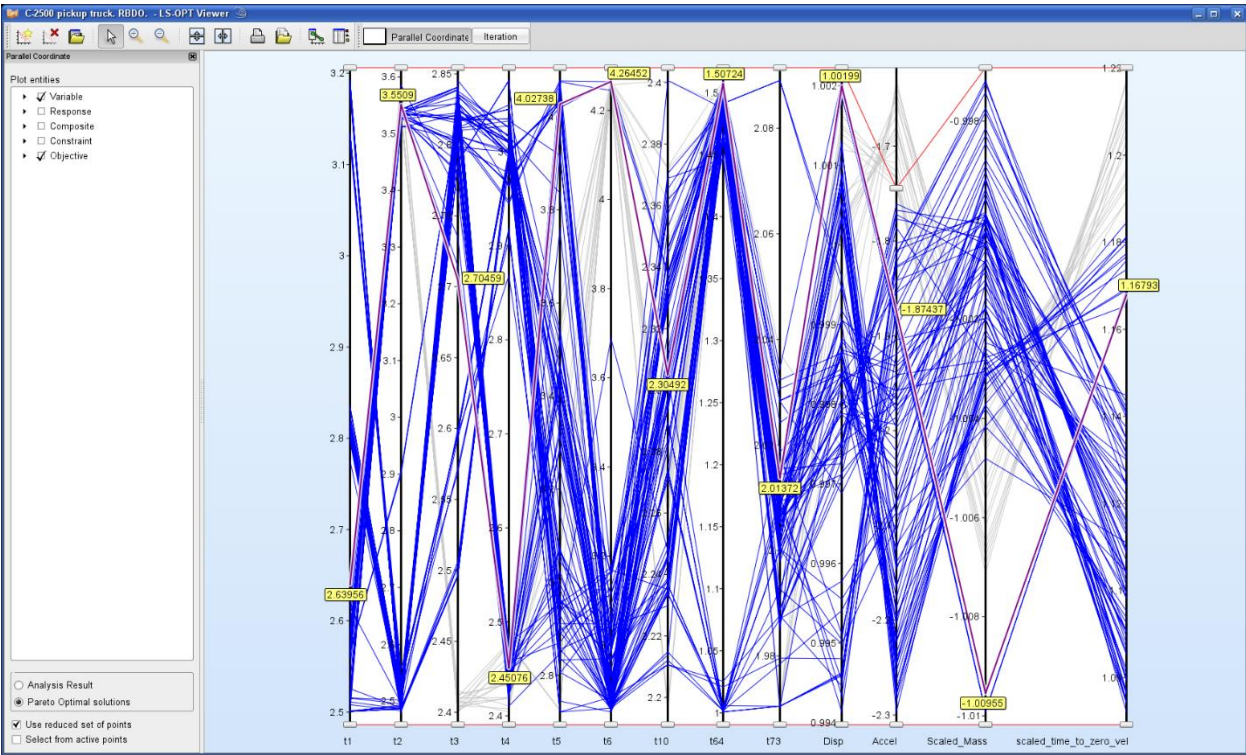
Figure 16-46: Parallel Coordinate Plot for Pareto optimal solutions with selected point (purple line)
