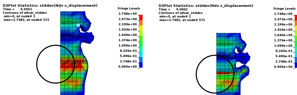
Figure 22-13: Tube Buckling – model with minimal x displacement (left) and maximal x displacement (right)
