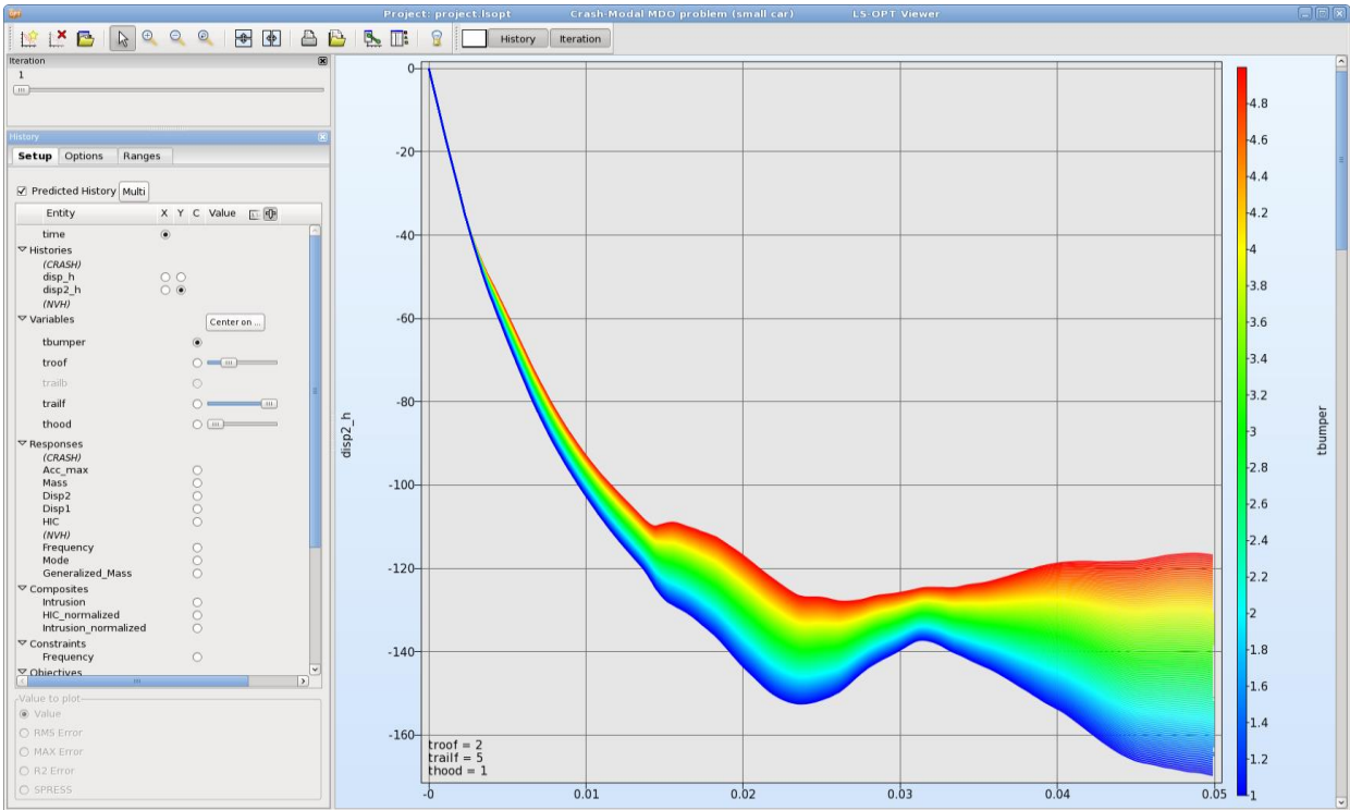
Figure 16-40: Predicted Histories colored by variable
