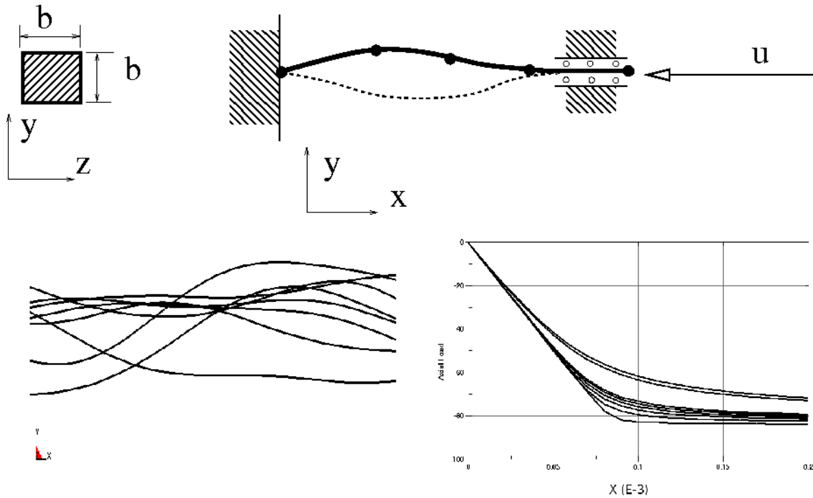
Figure 22-51: Problem with a stochastic field. The structural problem is shown in the top. In the bottom left are sample beams with the perturbation exaggerated by a factor 100, and the corresponding histories are shown in the bottom right.
