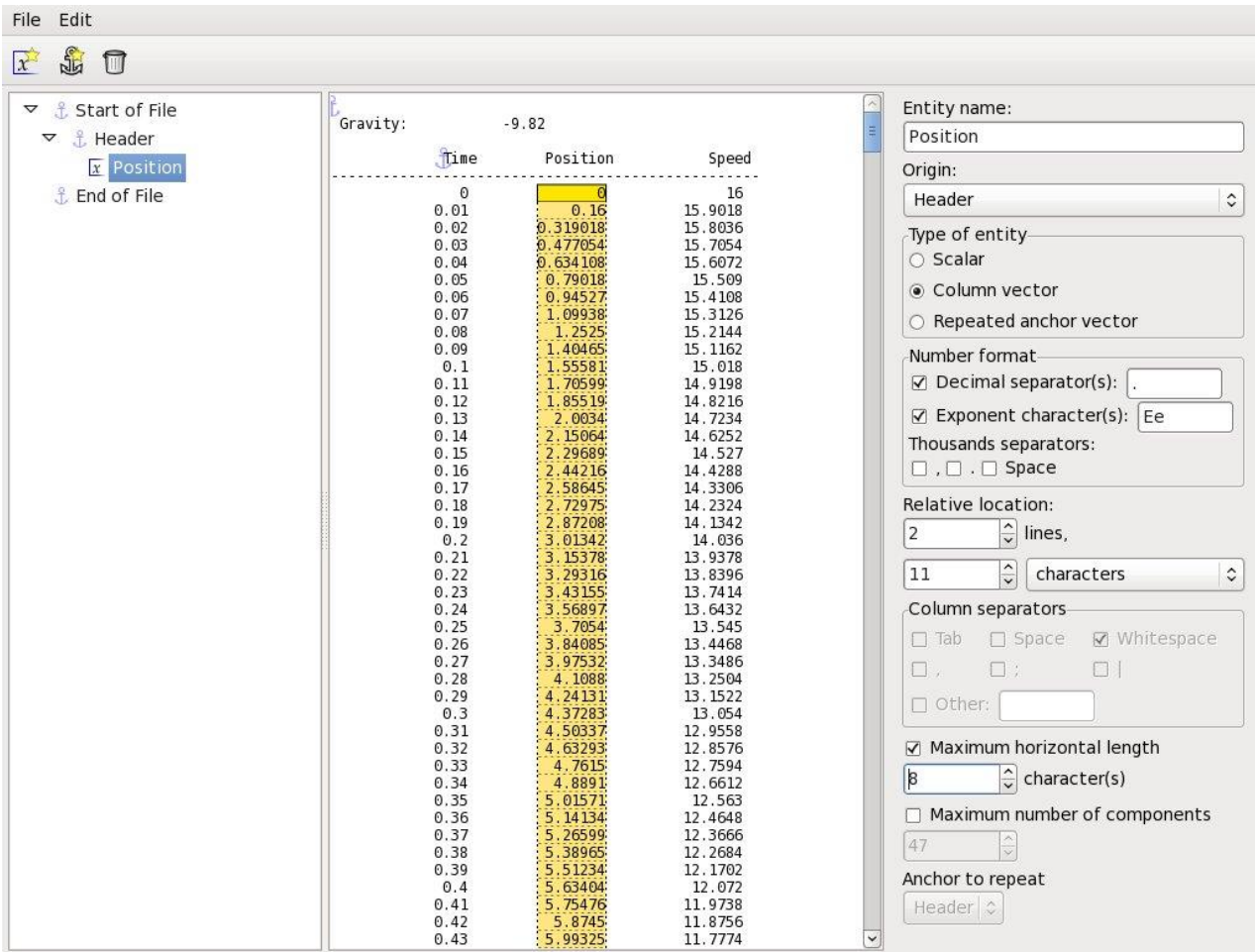
Figure 7-13: GenEx dialog; definition of a column vector entity
