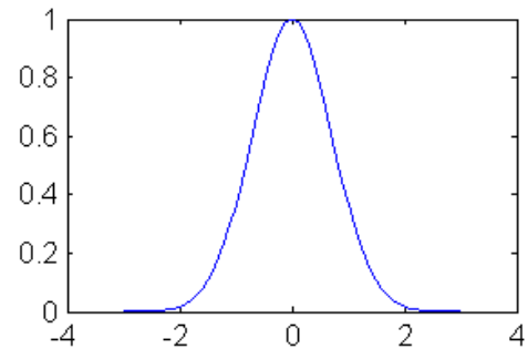
Figure 24-3: Radial basis transfer function y=\exp(-x^2)
