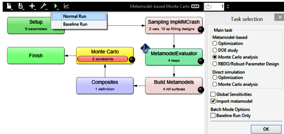
Figure 22-36: Monte Carlo analysis run with imported metamodel.
