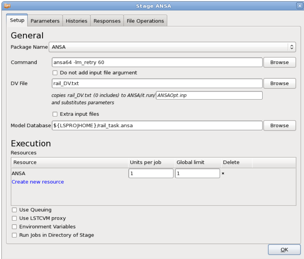
Figure 20-109: Stage dialog interfacing with ANSA
