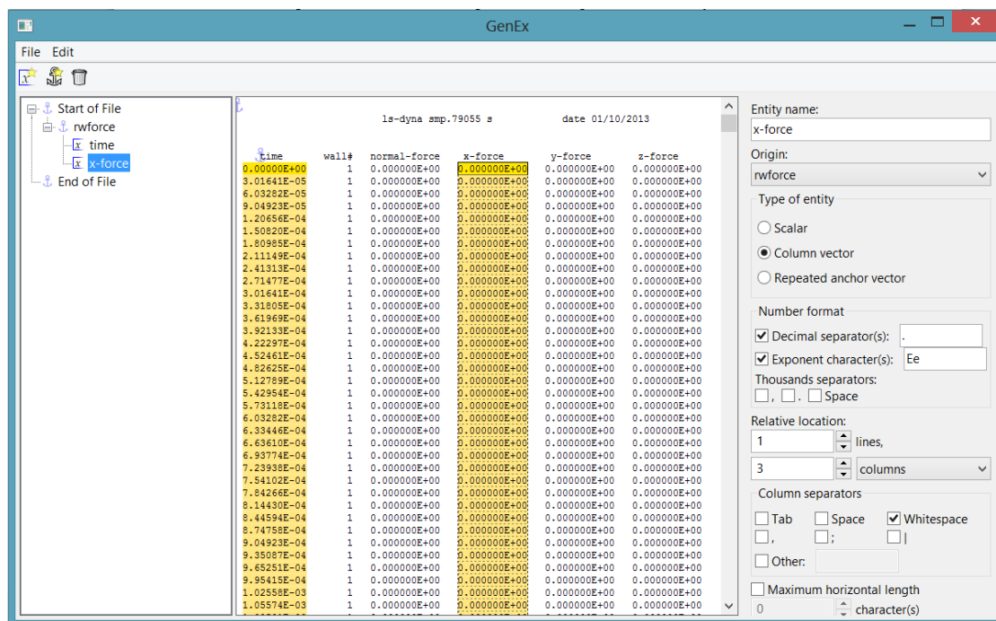
Figure 20-133: History definition using Column Vector as entity type
