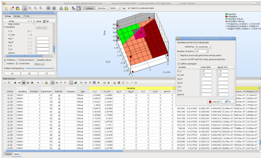
Figure 17-4: Generate virtual points: the dialog is shown for generating the points and the figure shows generated points on a metamodel surface.
