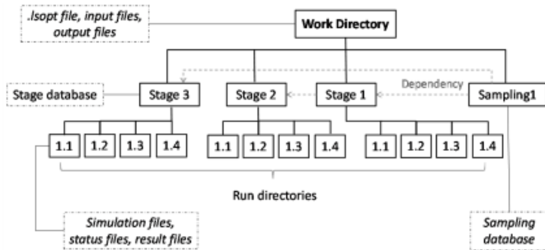
Figure E - 1: Directory structure in LS-OPT.
