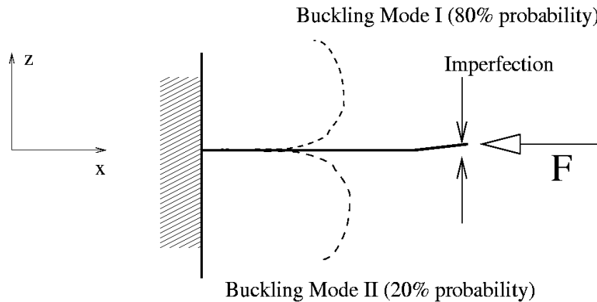
Figure 22-14: Plate Buckling Example
