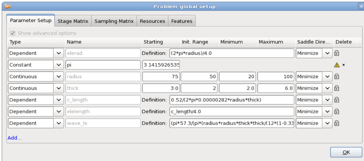
Figure 20-61: Parameter Setup: the length of the cylinder depending on the radius and the thickness is defined as a dependent to satisfy the mass constraint.
