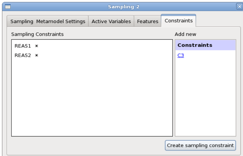
Figure 9-19: Definition of Sampling Constraints by selection from list or new creation.
