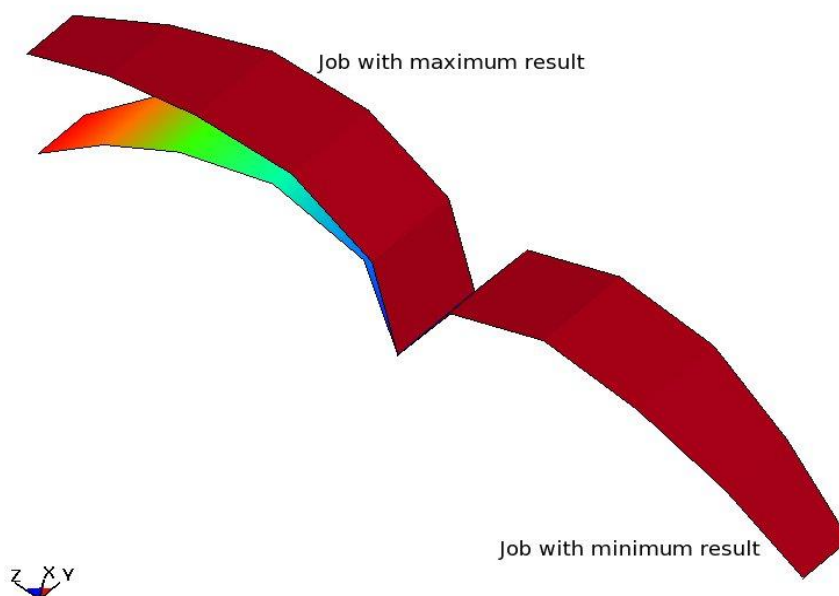
Figure 22-19: LS-OPT identified and displayed this bifurcation automatically using the GUI setting shown in the previous figure.
