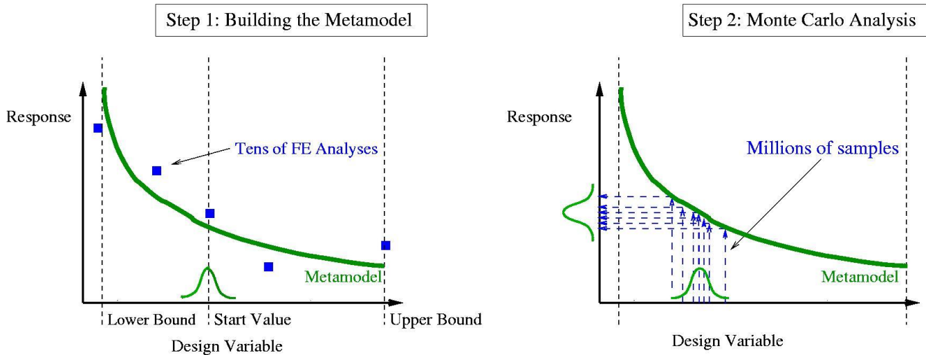
Figure 14-14: Metamodel-based Monte Carlo analysis. The method proceed in two steps: firstly a metamodel is created, and then the Monte Carlo simulation is done using the metamodel and the statistical distribution of the variable. Note that the metamodel for a design/control variable is constructed considering the upper and lower bound on the variable and not considering the statistical distribution. For a noise variable the upper and lower bounds for the creation of the metamodel are selected considering the statistical distribution.
