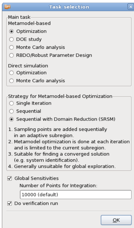
Figure 20-34: Task dialog; select Strategy Sequential with Domain Reduction
