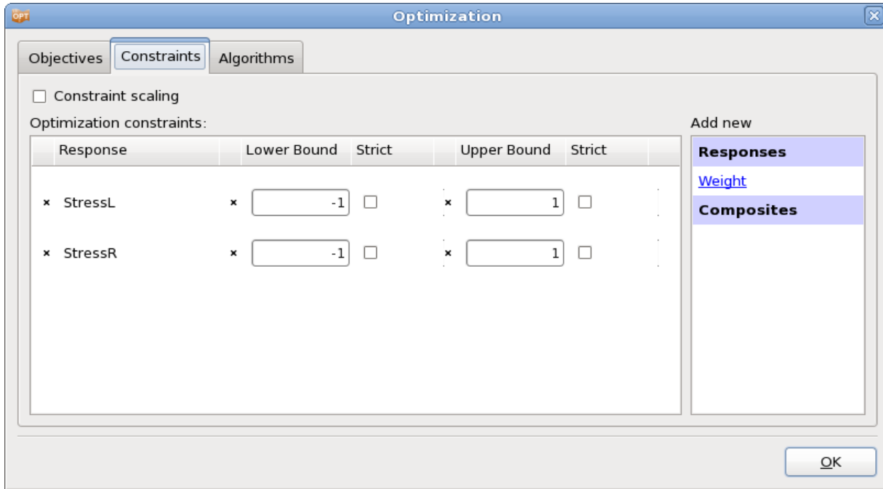
Figure 20-8: Constraints; select the respective responses from the list on the right and specify lower and upper bounds.
