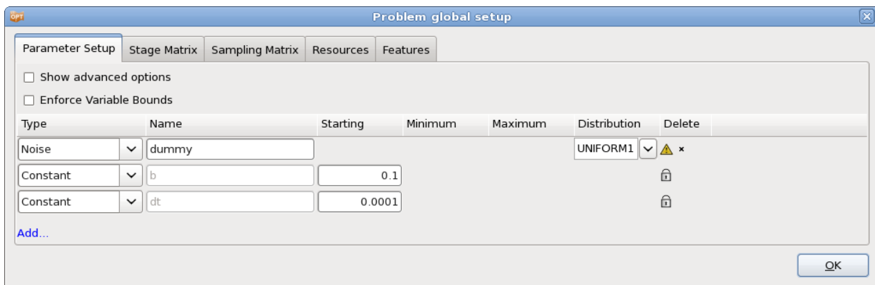
Figure 22-53: Parameter setup. Since the variable dummy is not used, an arbitrary distribution can be used here.
