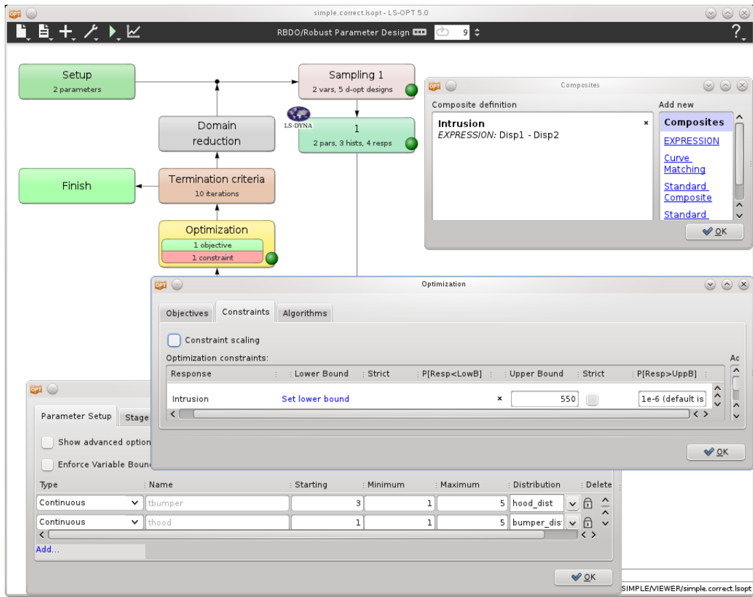
Figure 22-24: Probabilistic variable and constraint definition for RBDO
