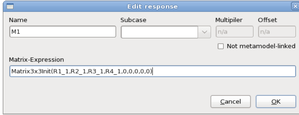
Figure 6-20: Matrix Expression: Initialization of a matrix
