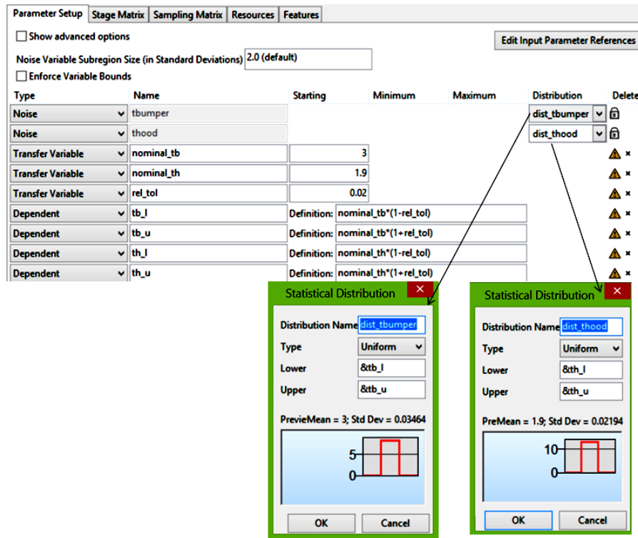
Figure 22-42: Variable distributions parameterized using Transfer Variables. These variables are treated as constants in the inner level Monte Carlo analysis, but may be optimization variable in an outer level (Section 19.7). The values of the Transfer Variables are set as the outer level samples variable values. Thus, for a specific outer level sample the Transfer Variables and their dependents (nominal variables and variable distribution ranges) are fixed, and the failure probabilities calculated in the inner level using these fixed distributions corresponds to that specific outer level sample.
