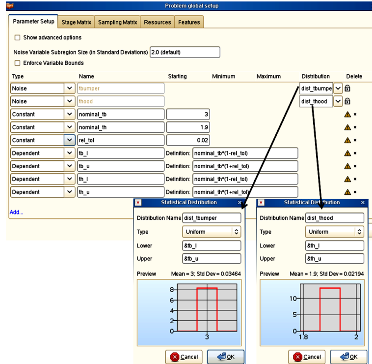
Figure 22-34: Parameterized variable distributions. As the distributions are parametrized, changing the values of the constants automatically updates the distributions.
