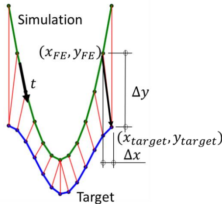
Figure 17-9: Contour mapping (Dynamic Time Warping example)
