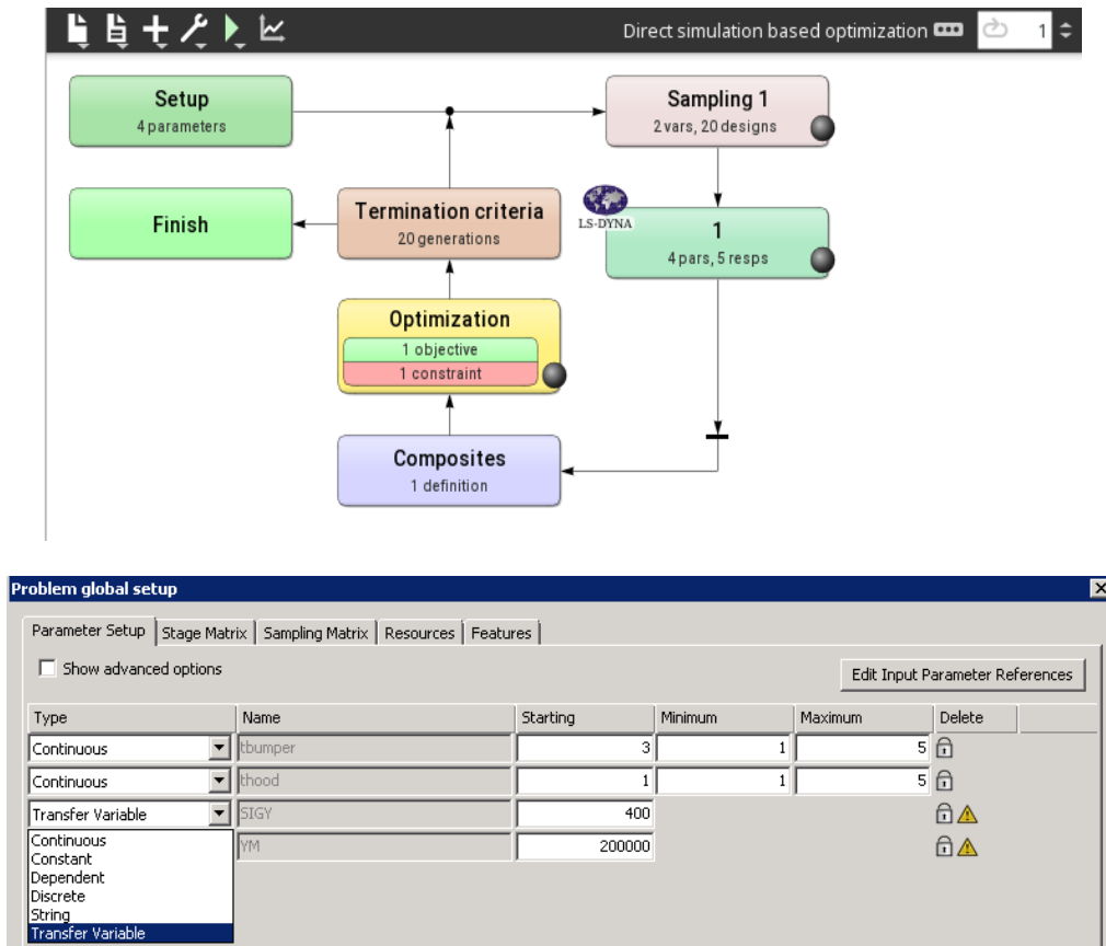
Figure 20-48: Multilevel Optimization inner level setup
