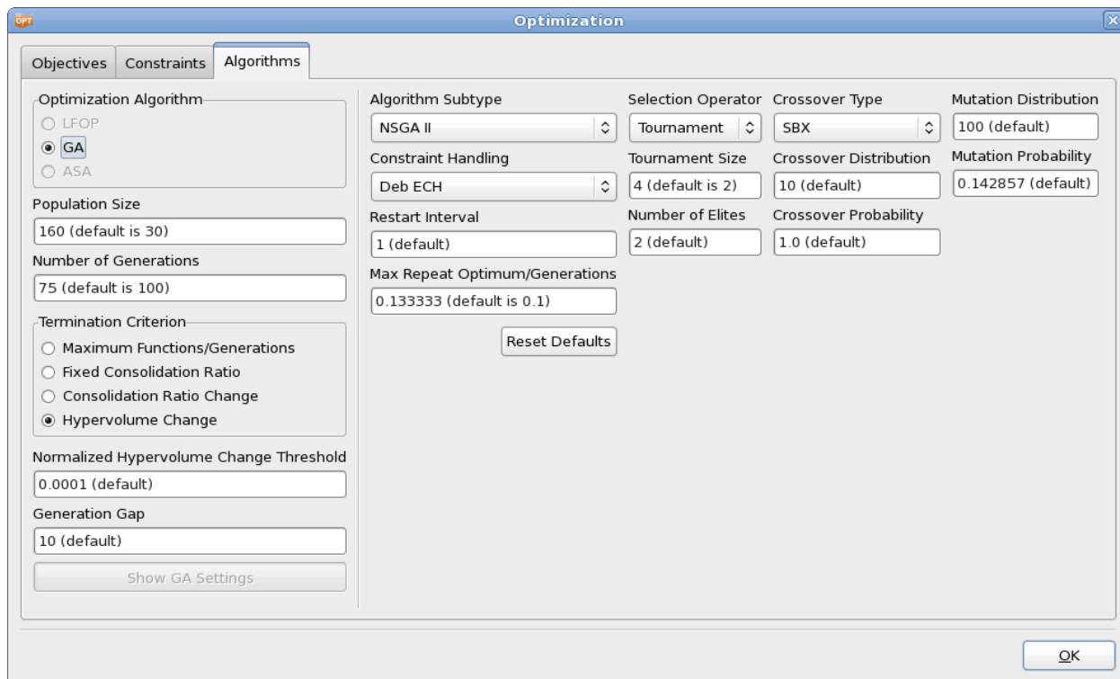
Figure 20-93: Options for Genetic Algorithm
