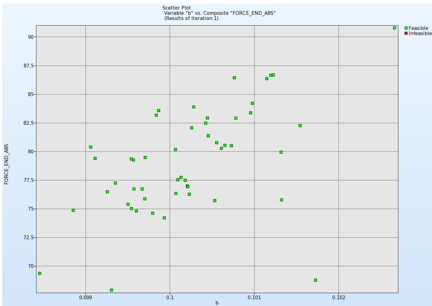
Figure 22-57: Plot of the responses using the thickness variable and a stochastic field.
