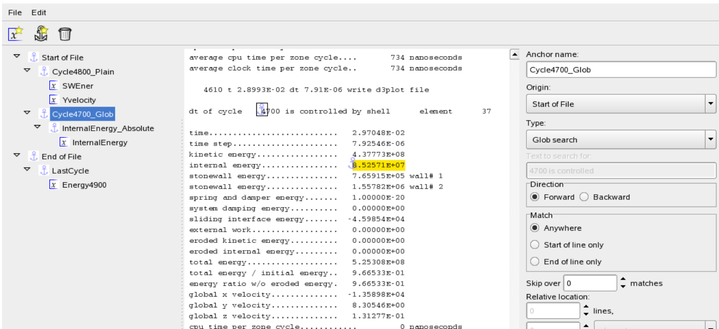
Figure 7-6: GenEx dialog; definition of an anchor
