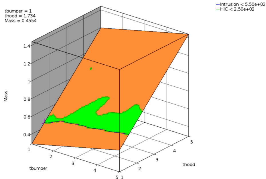
Figure 22-40: Surface plot of Mass. The green region is feasible. The magenta cross represents the optimum.
