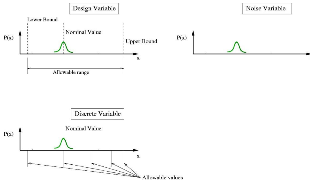
Figure 14-12: Probabilistic variables. The nominal value of a control variable can be adjusted by the optimization algorithm between the lower and upper bound; the probabilistic variation of a design variable is around this nominal value. A noise variable is described completely by the statistical distribution. A discrete variable, like design variable has a nominal value selected by the optimization algorithm; the probabilistic variation of the discrete variable is around this nominal value.
