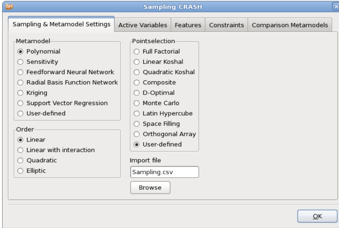
Figure 9-14: Sampling Dialog: User-defined point selection
