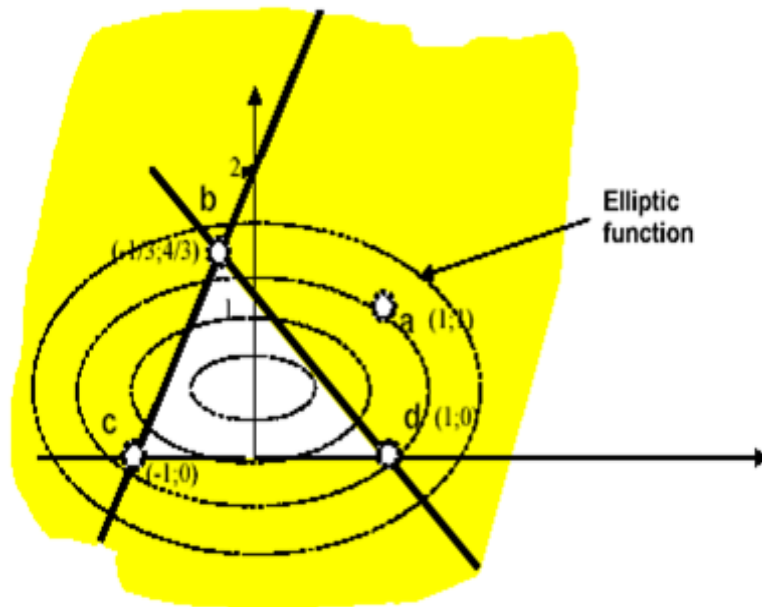
Figure 20-117: Objective and constraint functions.
