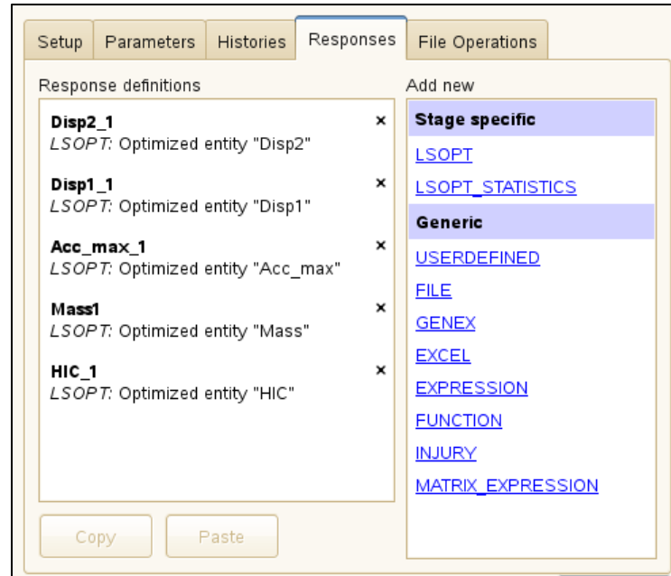
Figure 6-23: Main dialog for the extraction of LS-OPT stage responses. A special category (LSOPT STATISTICS) is available for statistical results produced by a Monte Carlo analysis.
