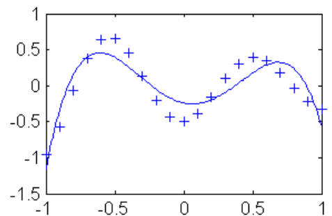
Figure 24-7: The same 21 data points as in Figure 24-5. Approximation with overlapping RBF neurons. The spread of RBF units is too high.
