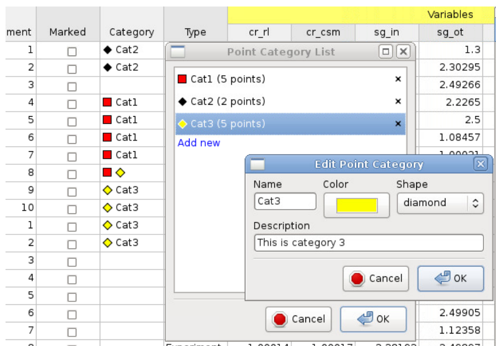
Figure 17-5: Point Categories dialog to define and manage Point Categories for user-defined coloring and plotting of points. Note that a design point can belong to multiple categories.
