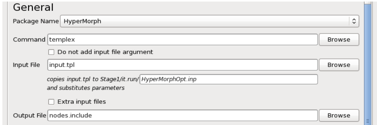
Figure 5-6: Stage Setup for HyperMorph
