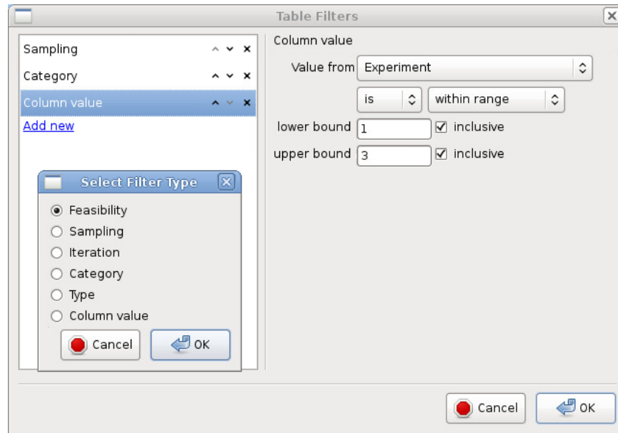
Figure 17-7: Manage filters dialog with 3 filters defined and a selection of new filter options.
