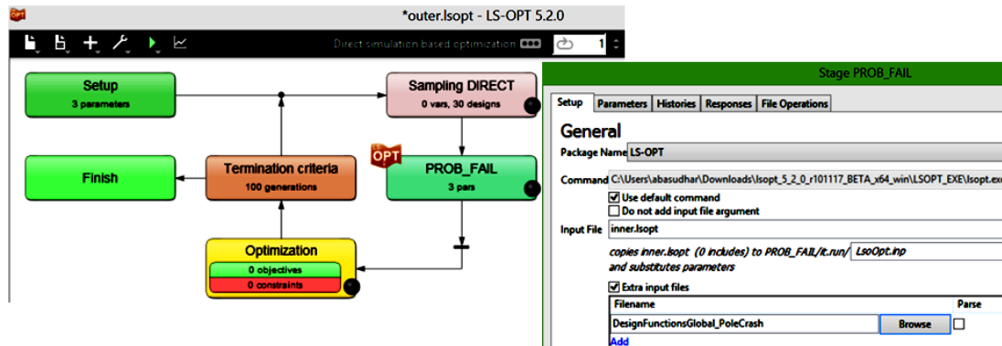
Figure 22-44: Outer level stage setup.
