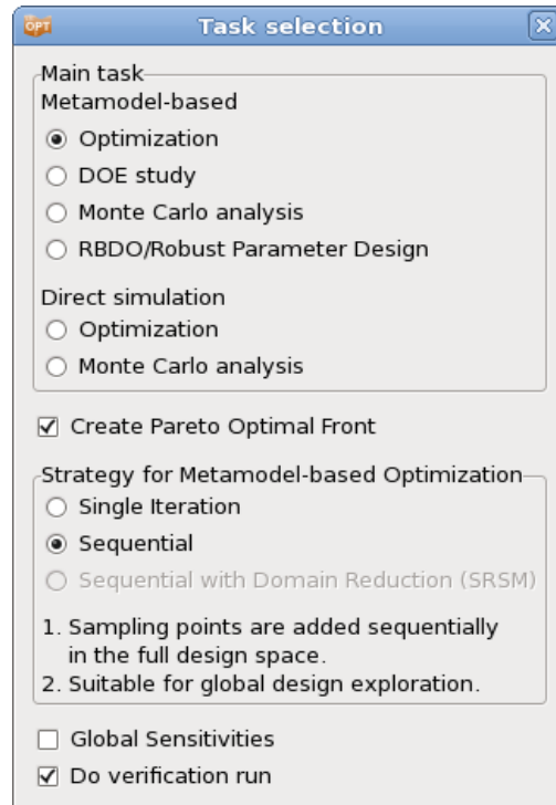
Figure 20-80: Task dialog; Calculating Pareto Optimal solutions using a metamodel-base method using sequential strategy.
