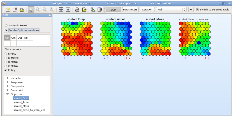
Figure 16-49: Self-Organizing Map, component plots of objectives
