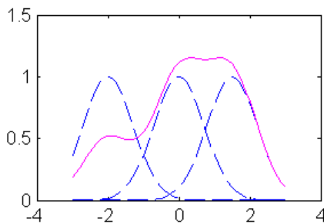
Figure 24-4: Weighted sum of radial basis transfer functions. Three radial basis functions (dashed lines) are scaled and summed to produce a function (solid line).
