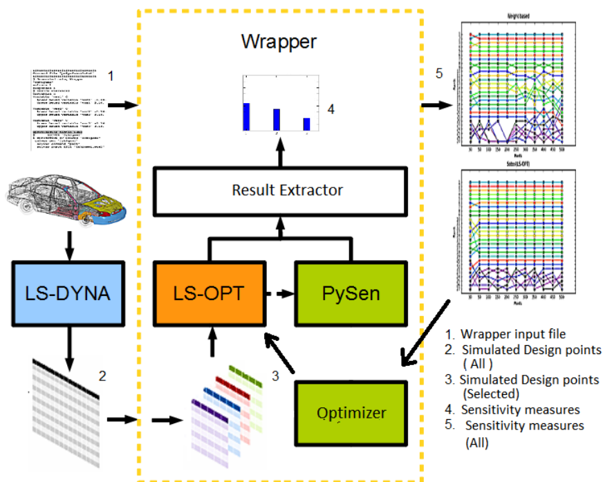
Fig. 4: Test system
