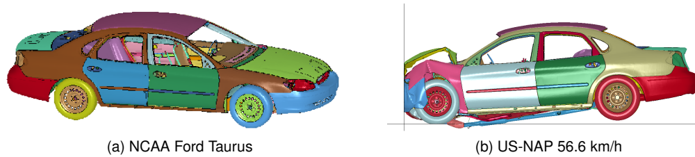
Fig. 5: Crash test example (courtesy of [2])
