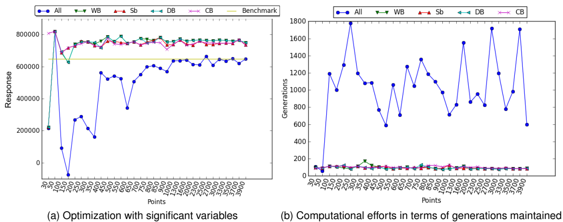
Fig. 7: Optimization results for US-NAP
