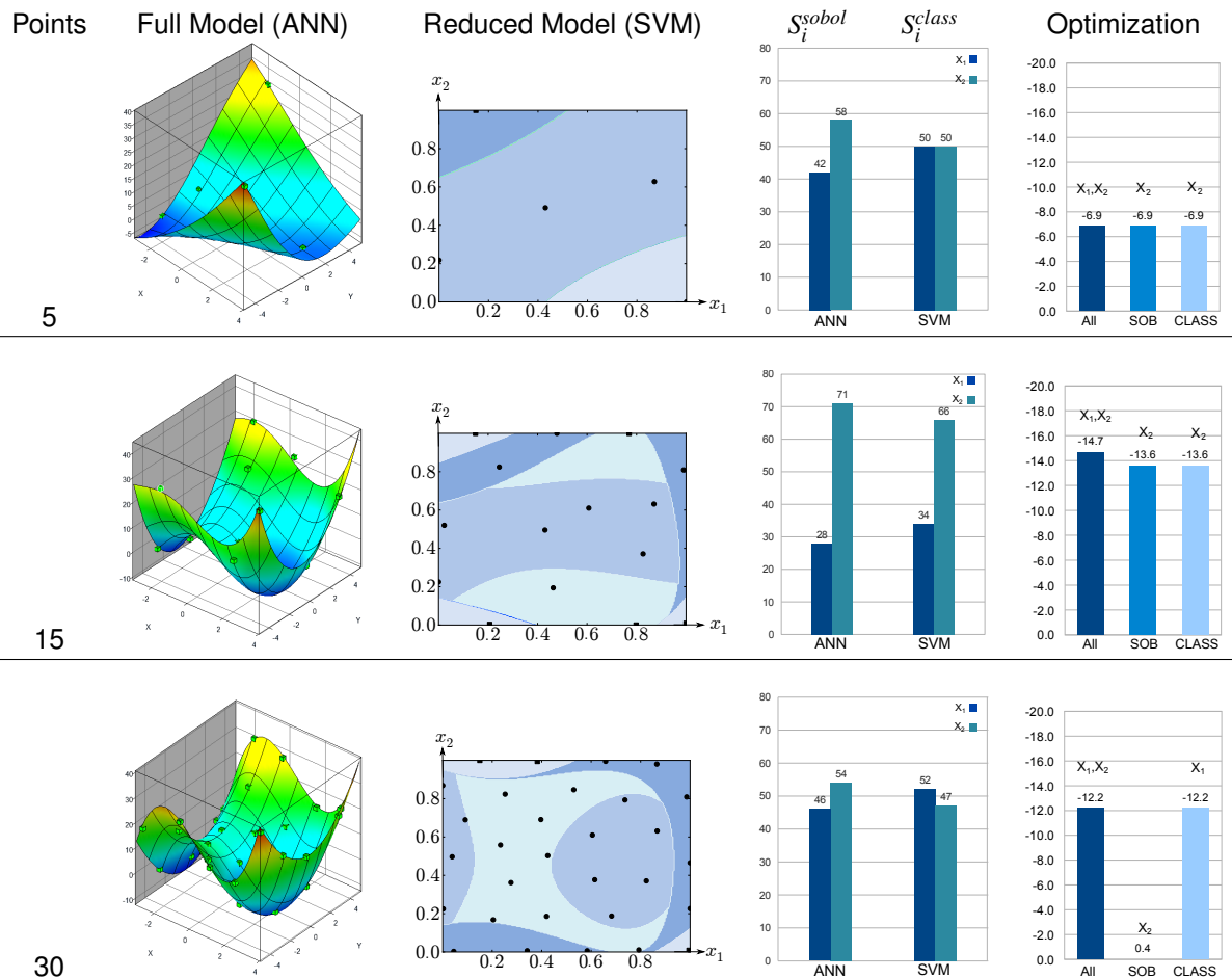
Fig. 2: Optimization of example function
