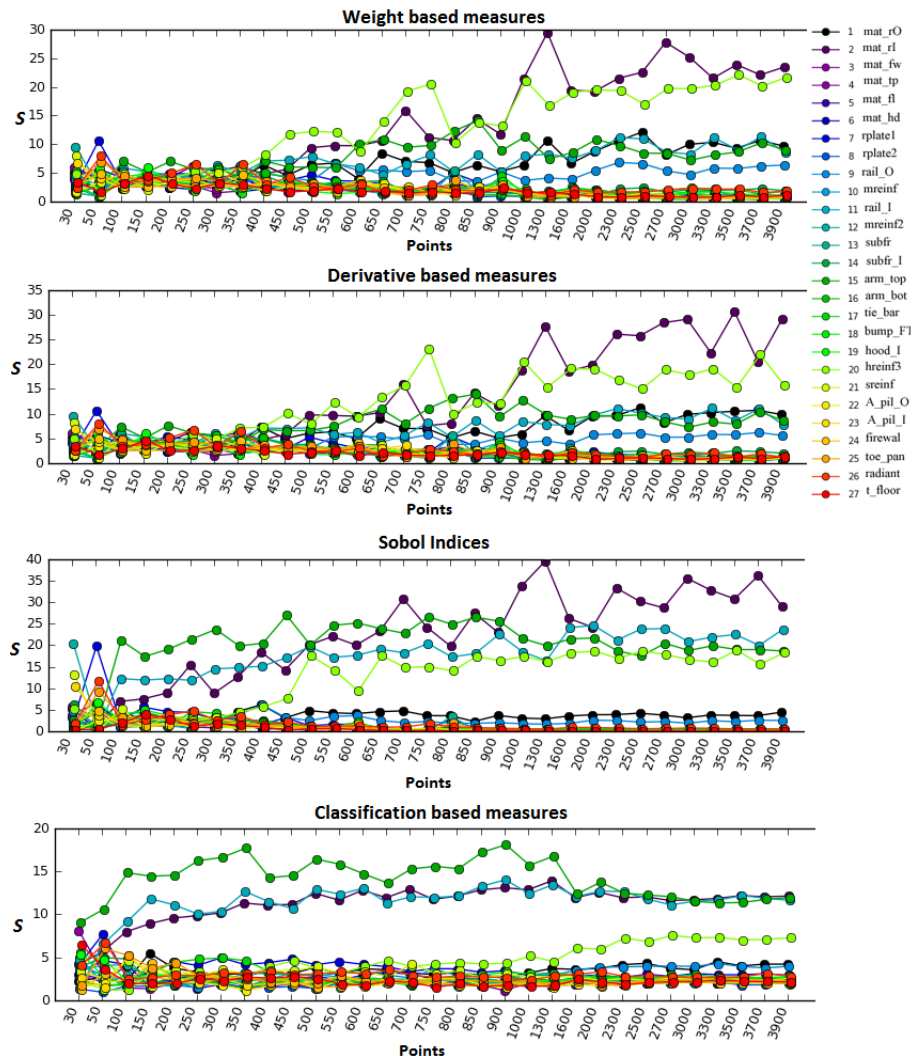
Fig. 6: Sensitivity results for US-NCAP [10]
