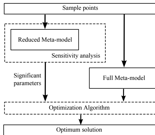
Fig. 3: Optimization with reduced meta-models
